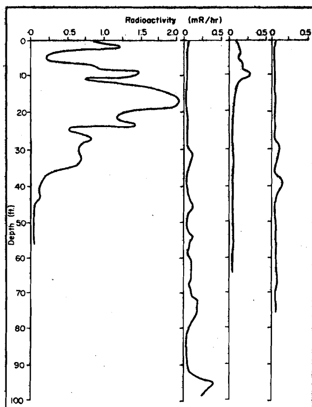
FIGURE 12. Four examples of radiometric well logs from drill holes on the Silver Queen claim (Locality SU-3), Esmeralda County.
