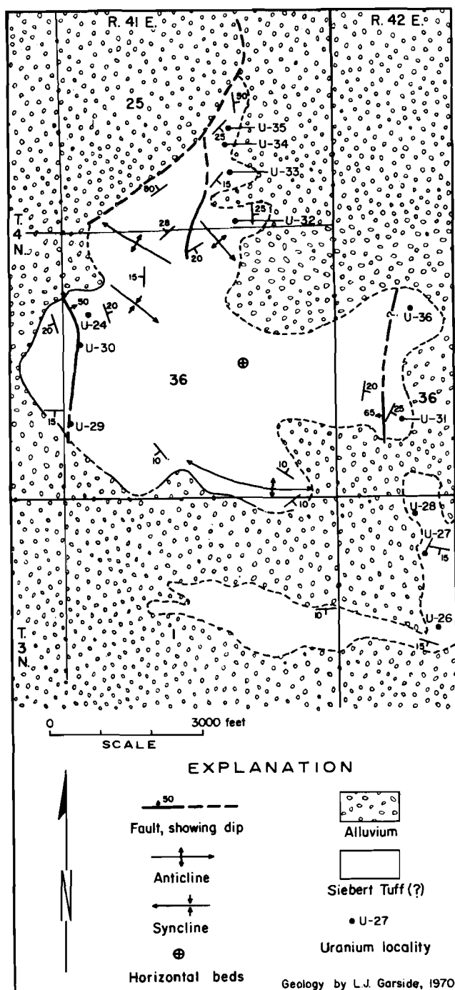
FIGURE 26. Uranium occurrences in the Tonopah area, Nye County.
