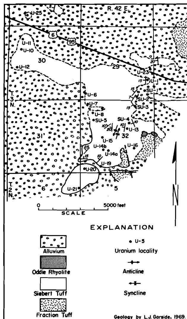
FIGURE 10. Uranium occurrences in the part of Esmeralda County adjacent to Tonopah.
