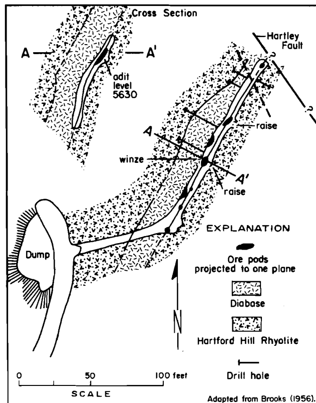
FIGURE 30. Geology and underground workings of the DeLongchamps prospect, Washoe County.
