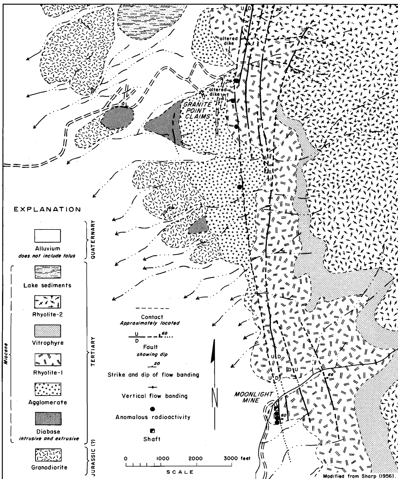
FIGURE 14. Geologic map of the vicinity of the Moonlight mine and Granite Point claims, Kings River area, Humboldt County.
