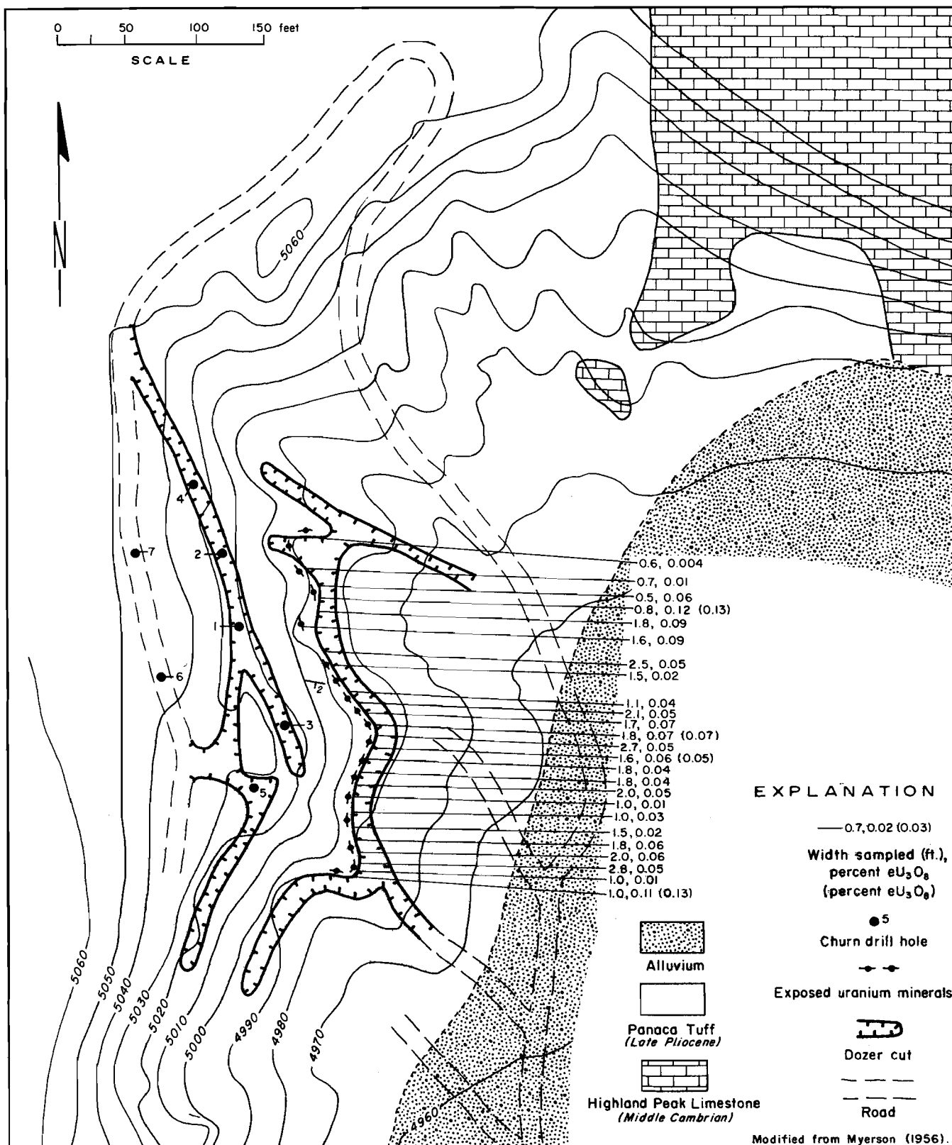
FIGURE 21. Geologic and assay map of the White Cloud prospect, Lincoln County. Widths and grades of the more significant samples are shown.
