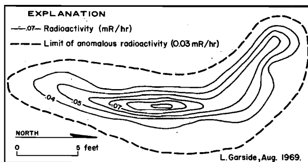
FIGURE 11. Radioactivity isolines at Locality U-10, in Esmeralda County near Tonopah.
