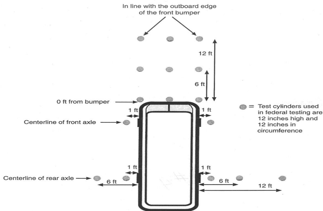
Figure SL1-2. Federal Mirror Field of Vision Test
