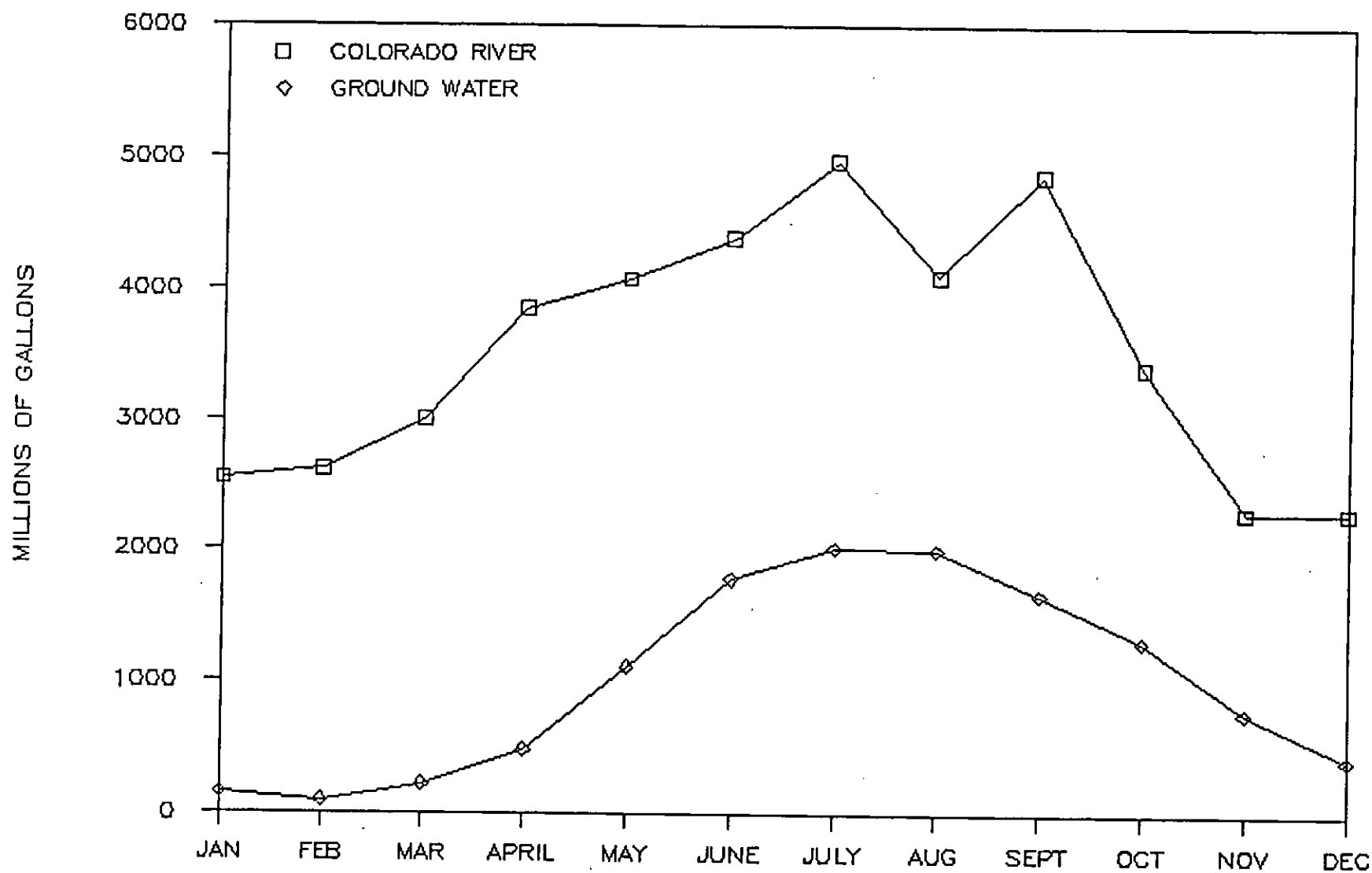
Figure 2. Las Vegas Valley Water District Ground-Water And Imported Colorado River Water Usage For 1987
