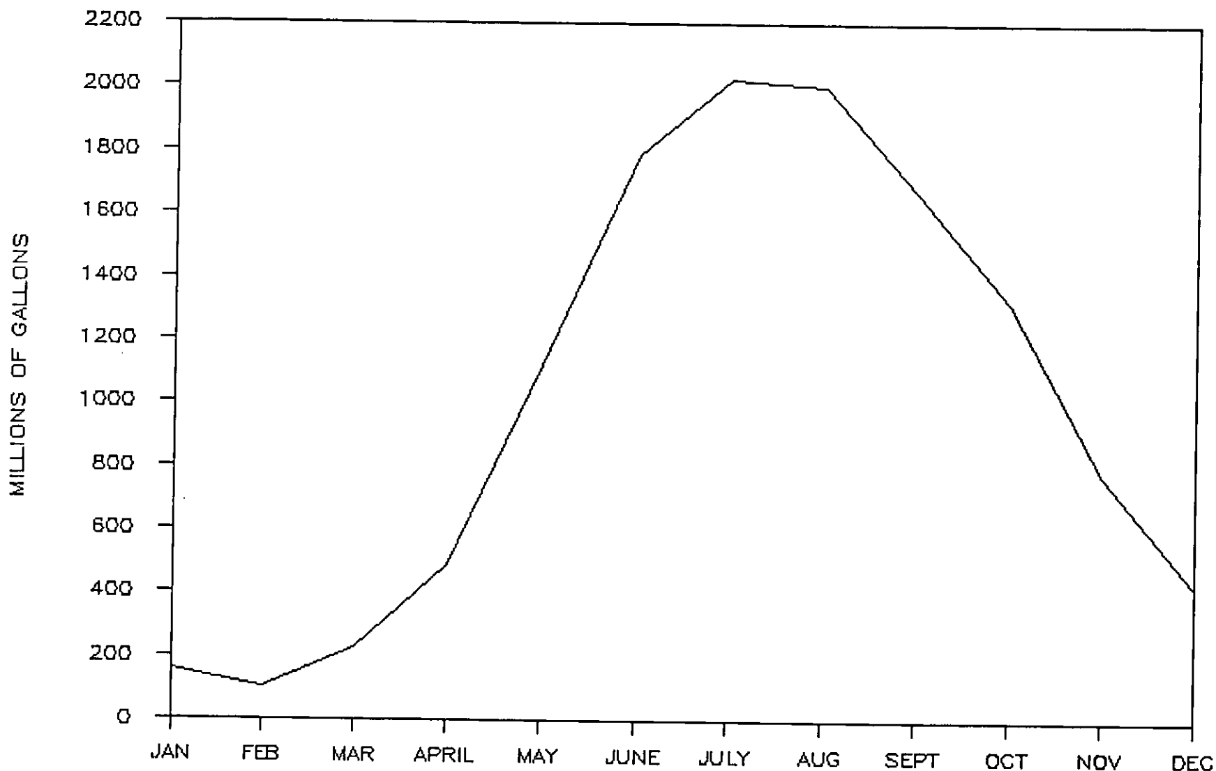
Figure 1. Las Vegas Valley Water District Monthly Well Production For 1987
