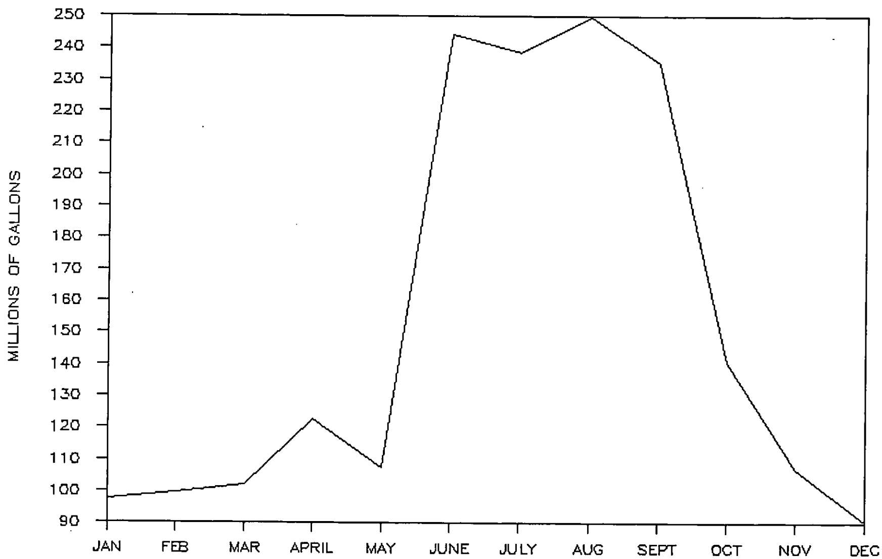
Figure 3. City of North Las Vegas Monthly Well Production For 1987
