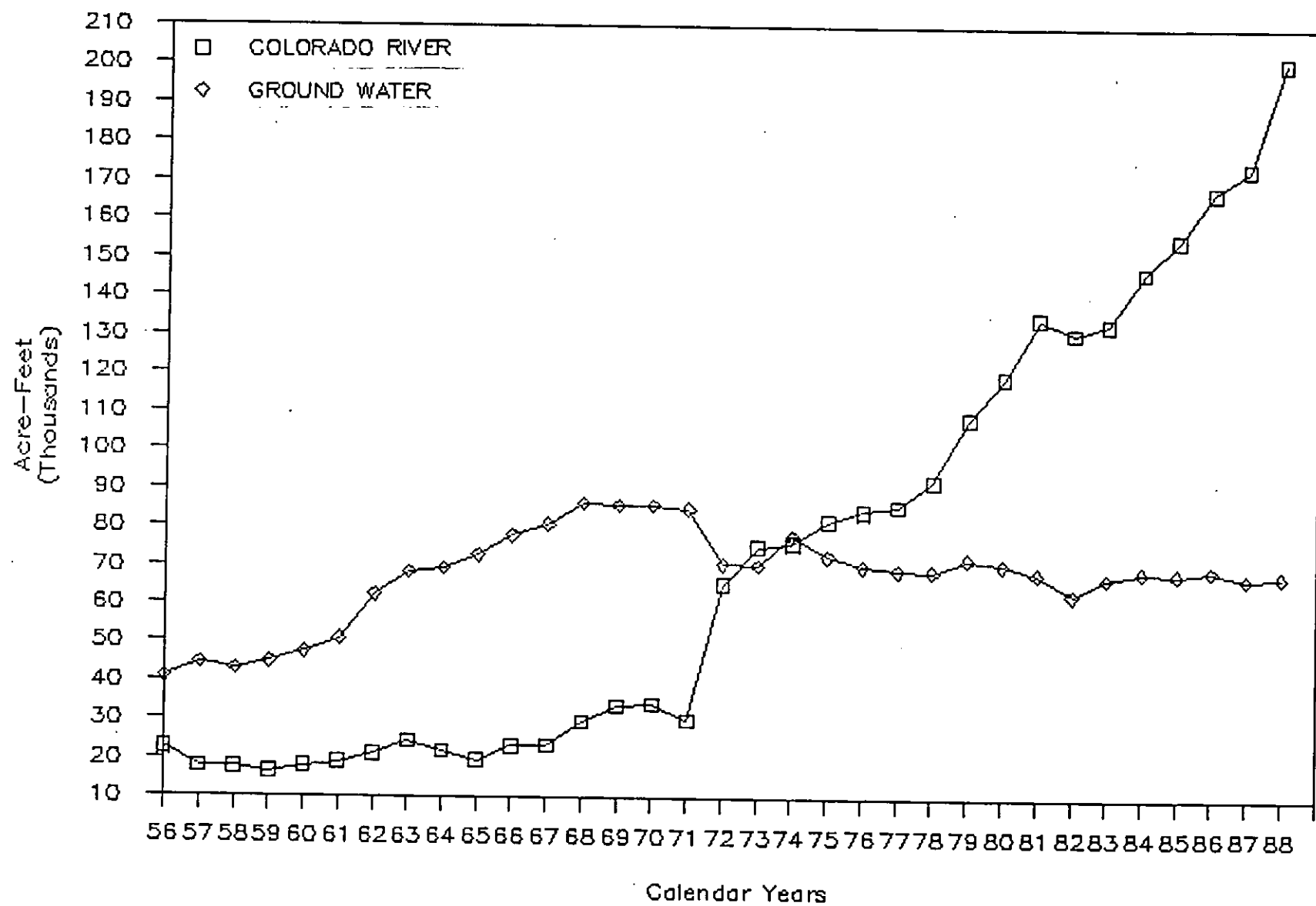
Figure 7. Total ground-water and Colorado River water usage for the Las Vegas Valley Basin, 1956-1988
