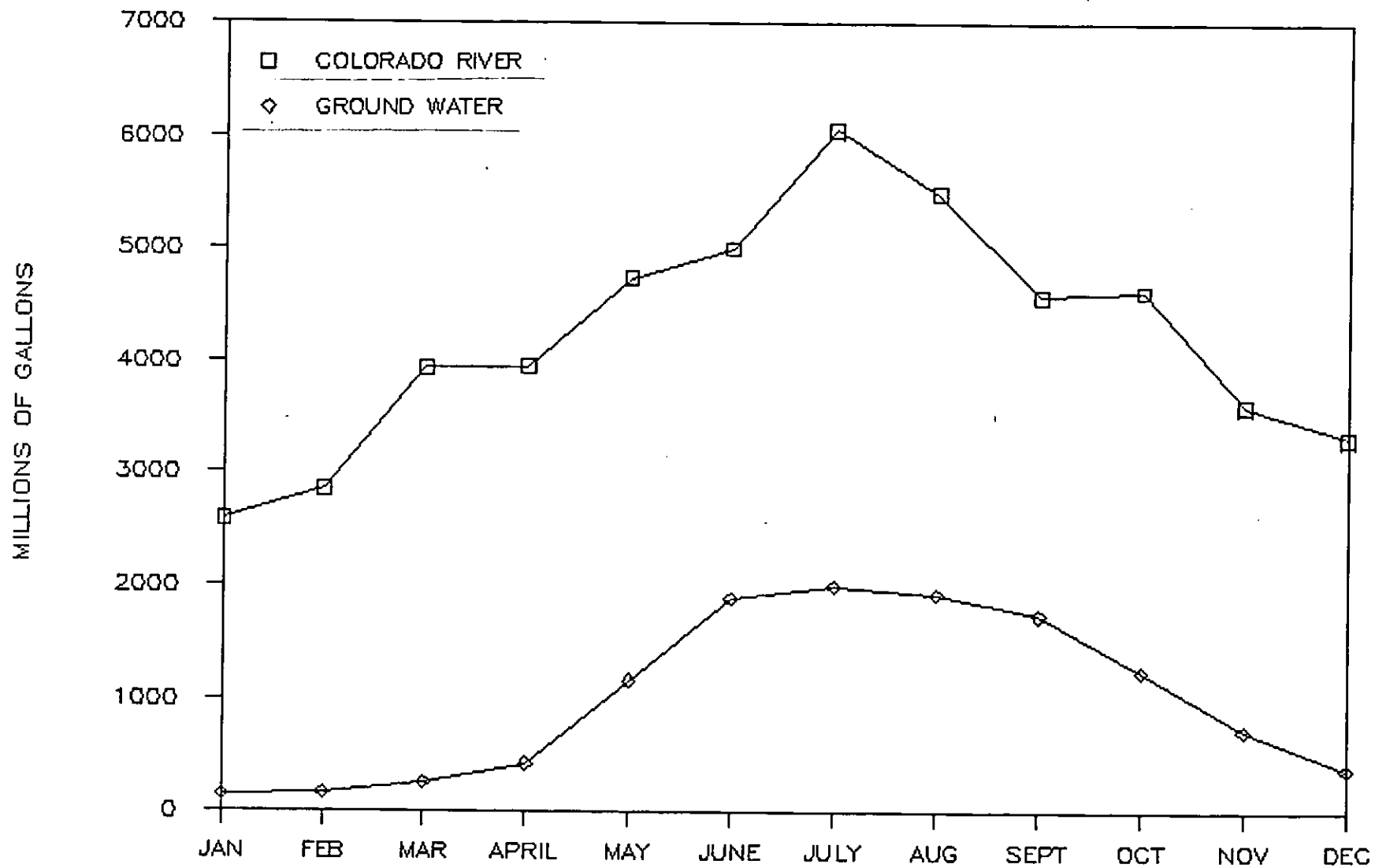
Figure 2. Las Vegas Valley Water District ground-water and Colorado River water usage for 1988
