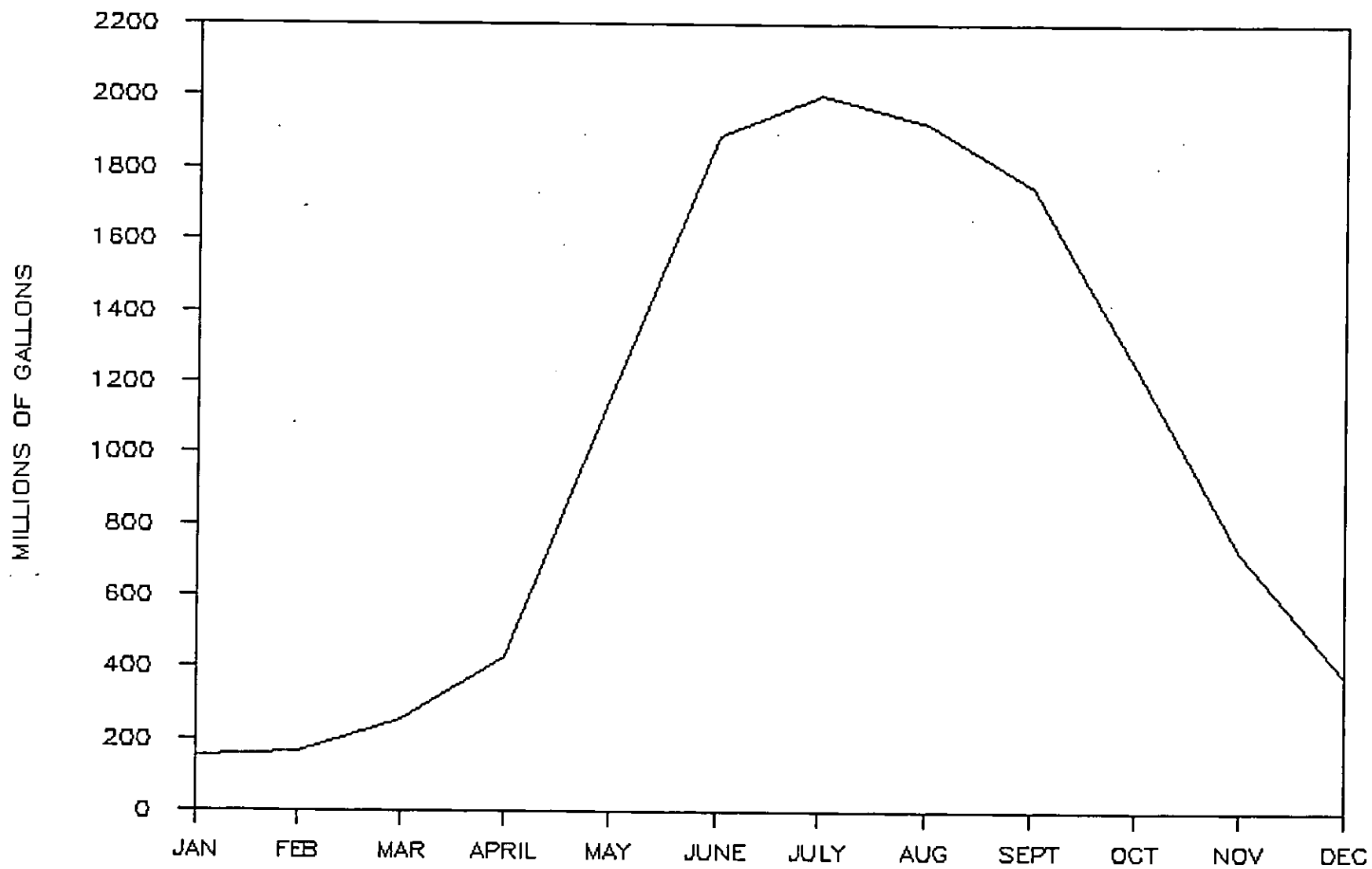
Figure 1. Las Vegas Valley Water District monthly well production for 1988
