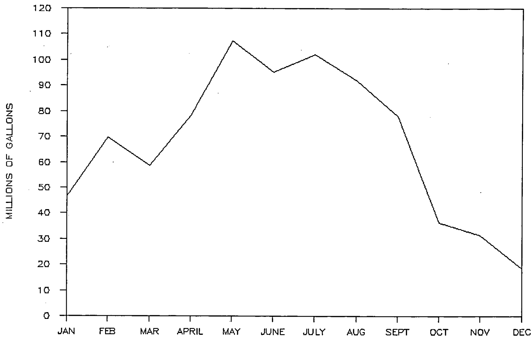
Figure 5. Nellis Air Force Base monthly well production for 1988
