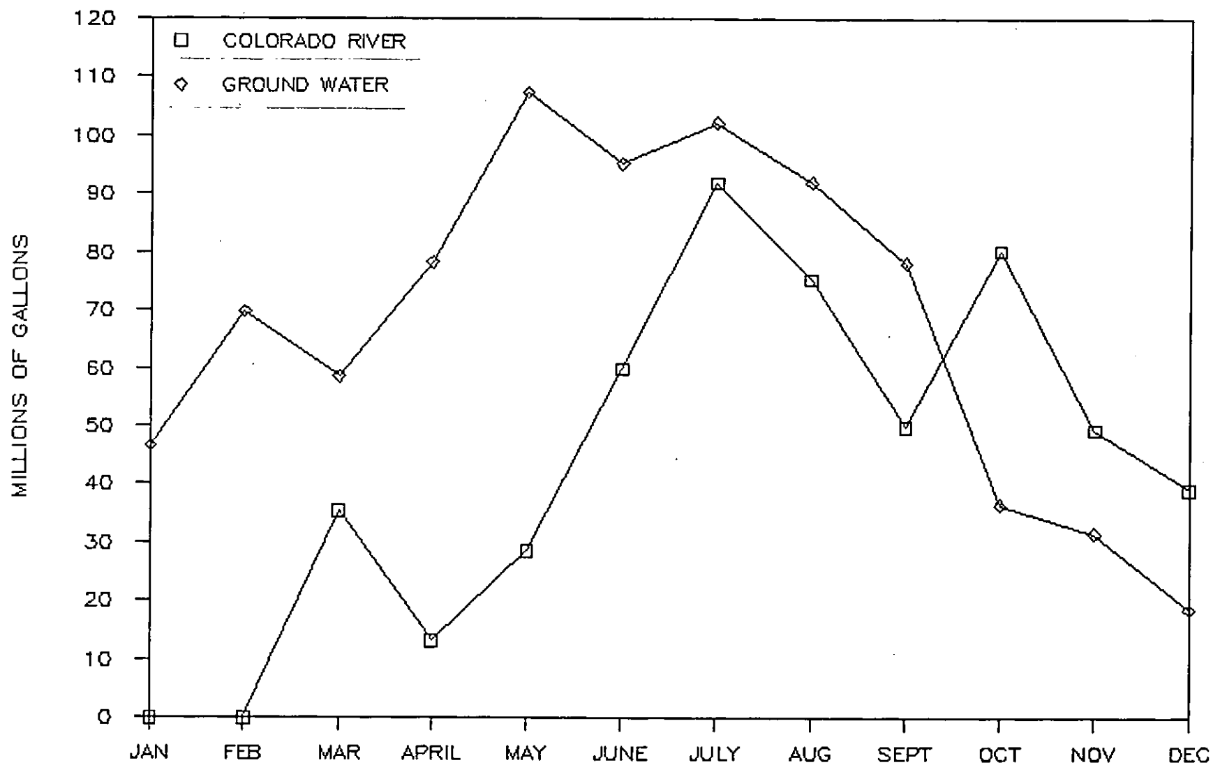
Figure 6. Nellis Air Force Base ground-water and imported Colorado River water usage for 1988
