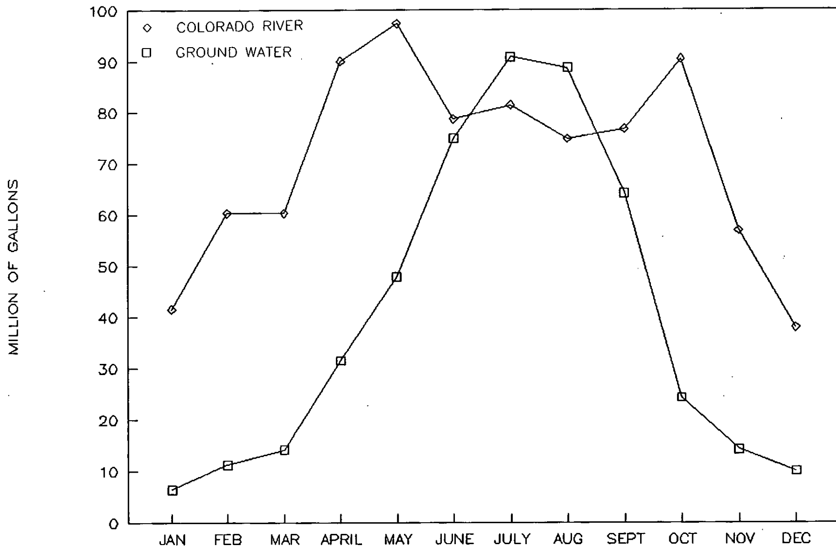
Figure 6. Nellis Air Force Base ground-water and imported Colorado River water usage for 1991
