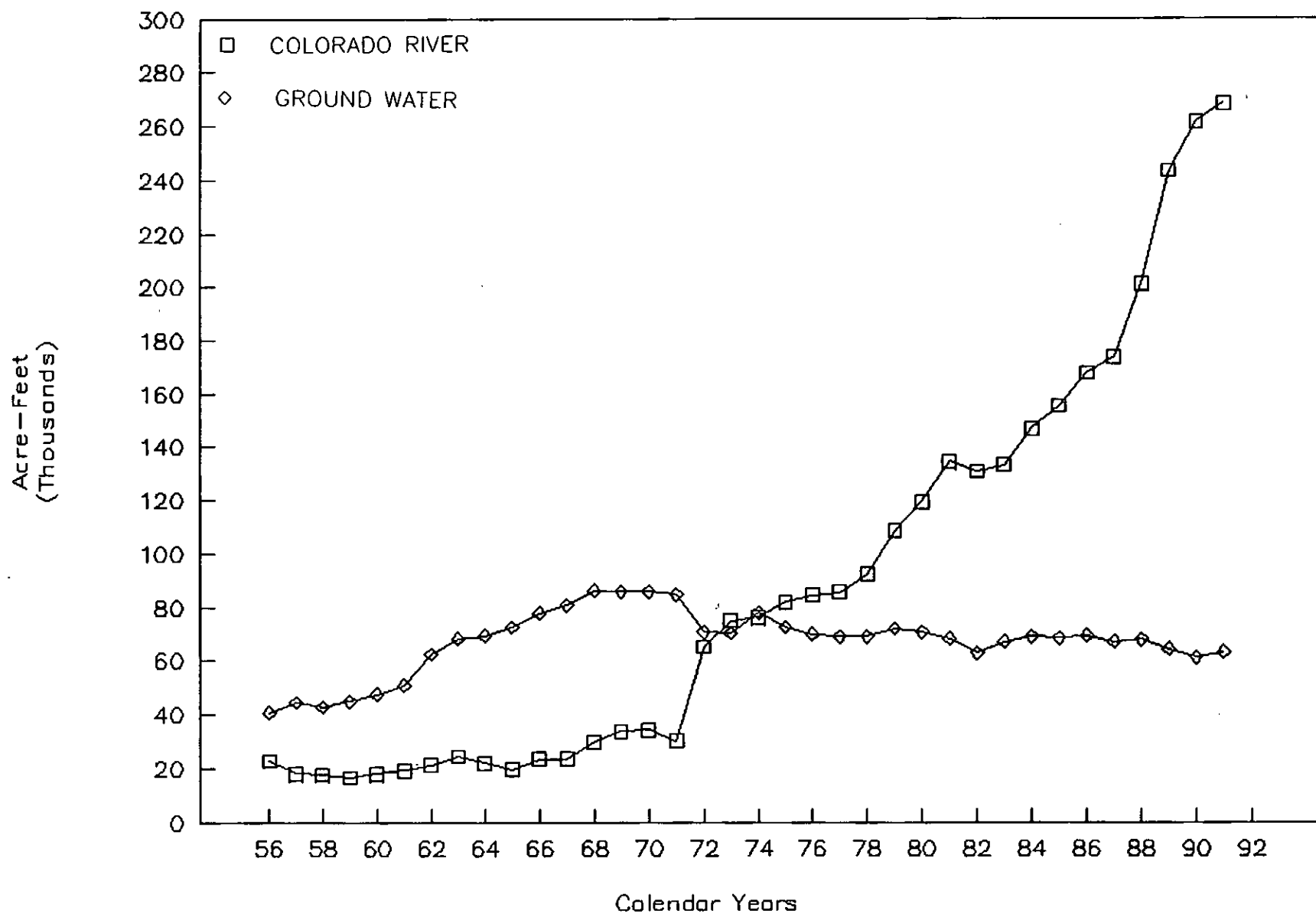
Figure 7. Total ground-water and Colorado River water usage for the Las Vegas Valley Basin, 1956-1991
