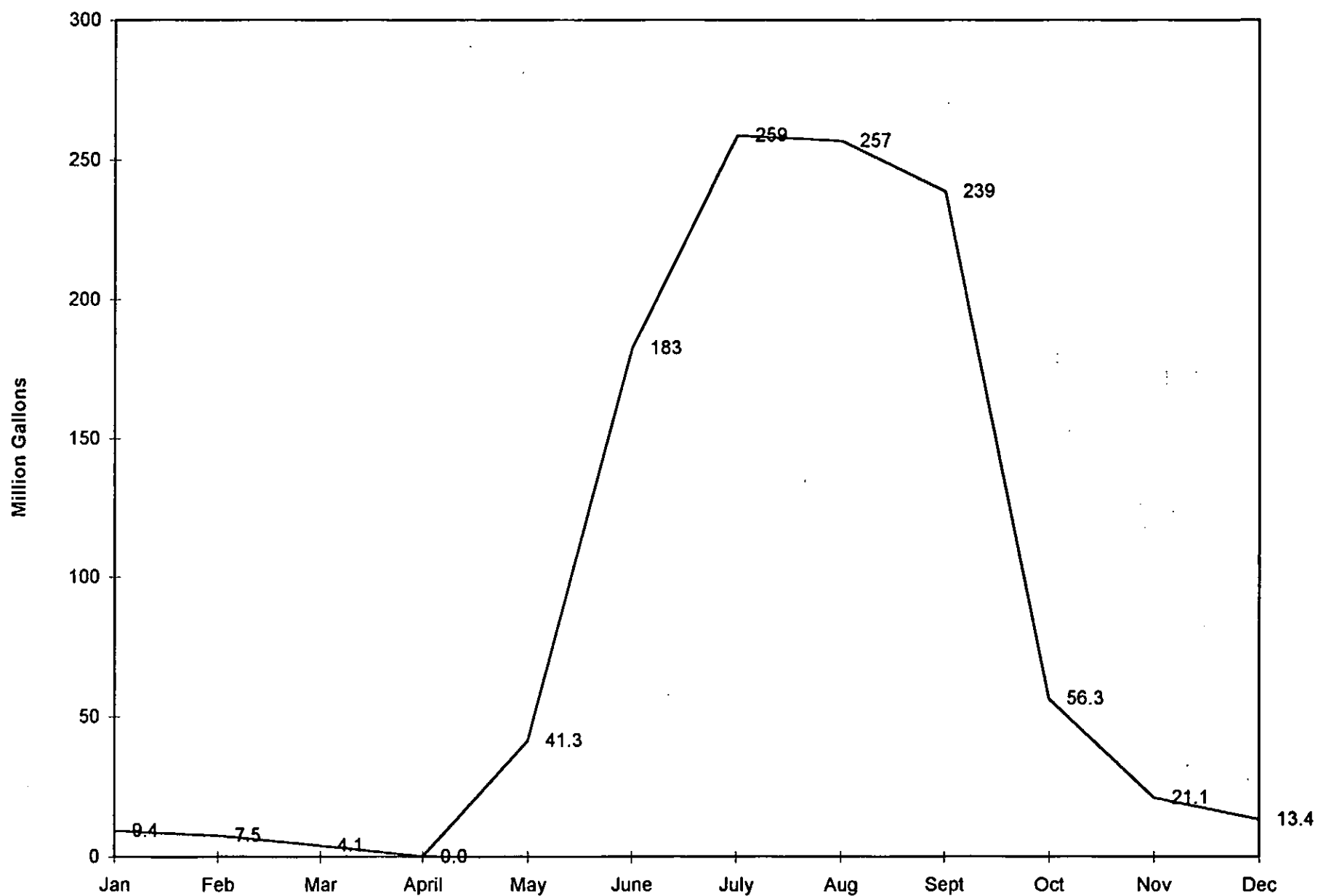
Figure 3. City of North Las Vegas monthly well production for 1995.
