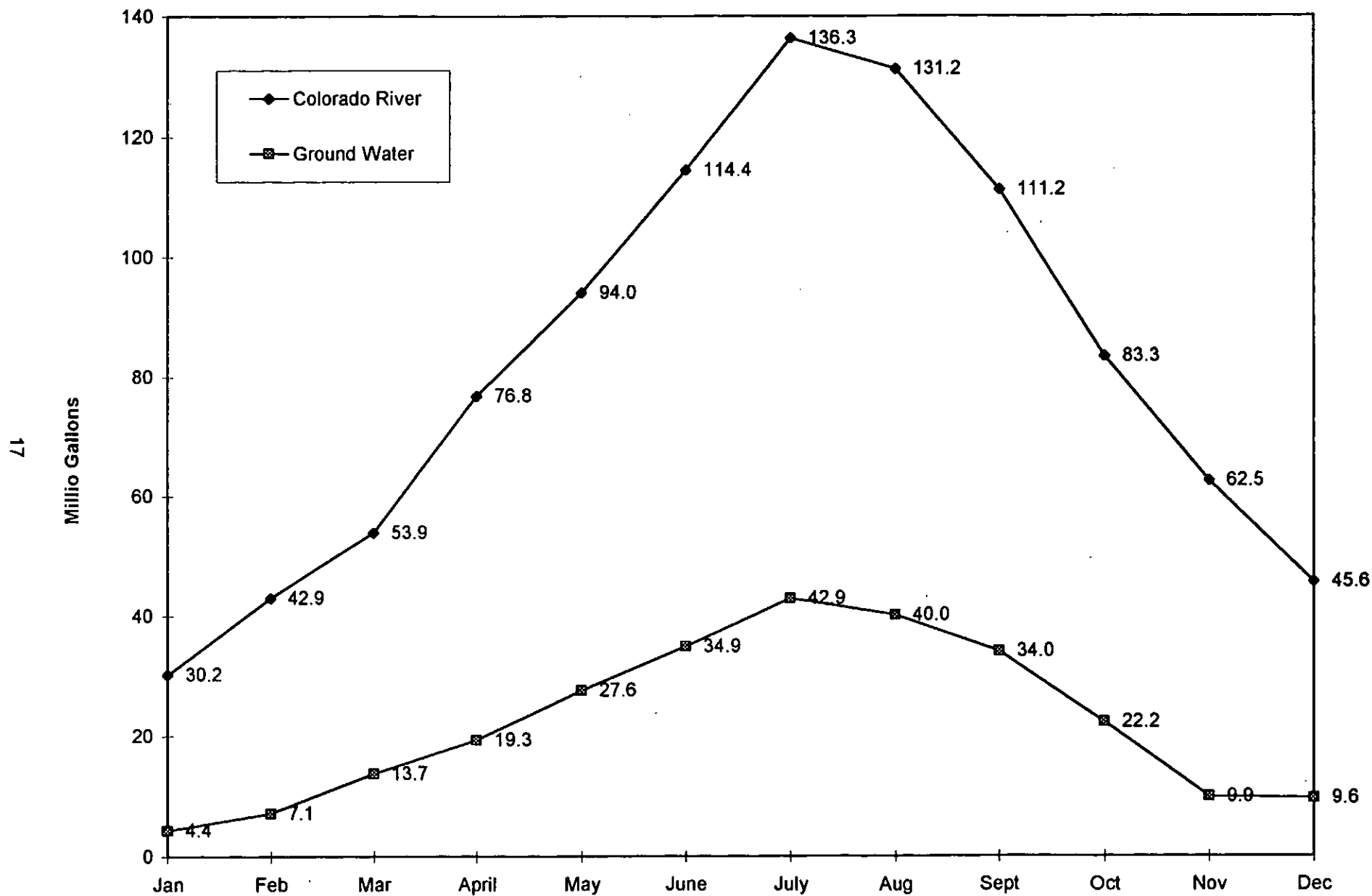
Figure 6. Nellis Air Force Base Ground Water and imported Colorado River water usage for 1995.
