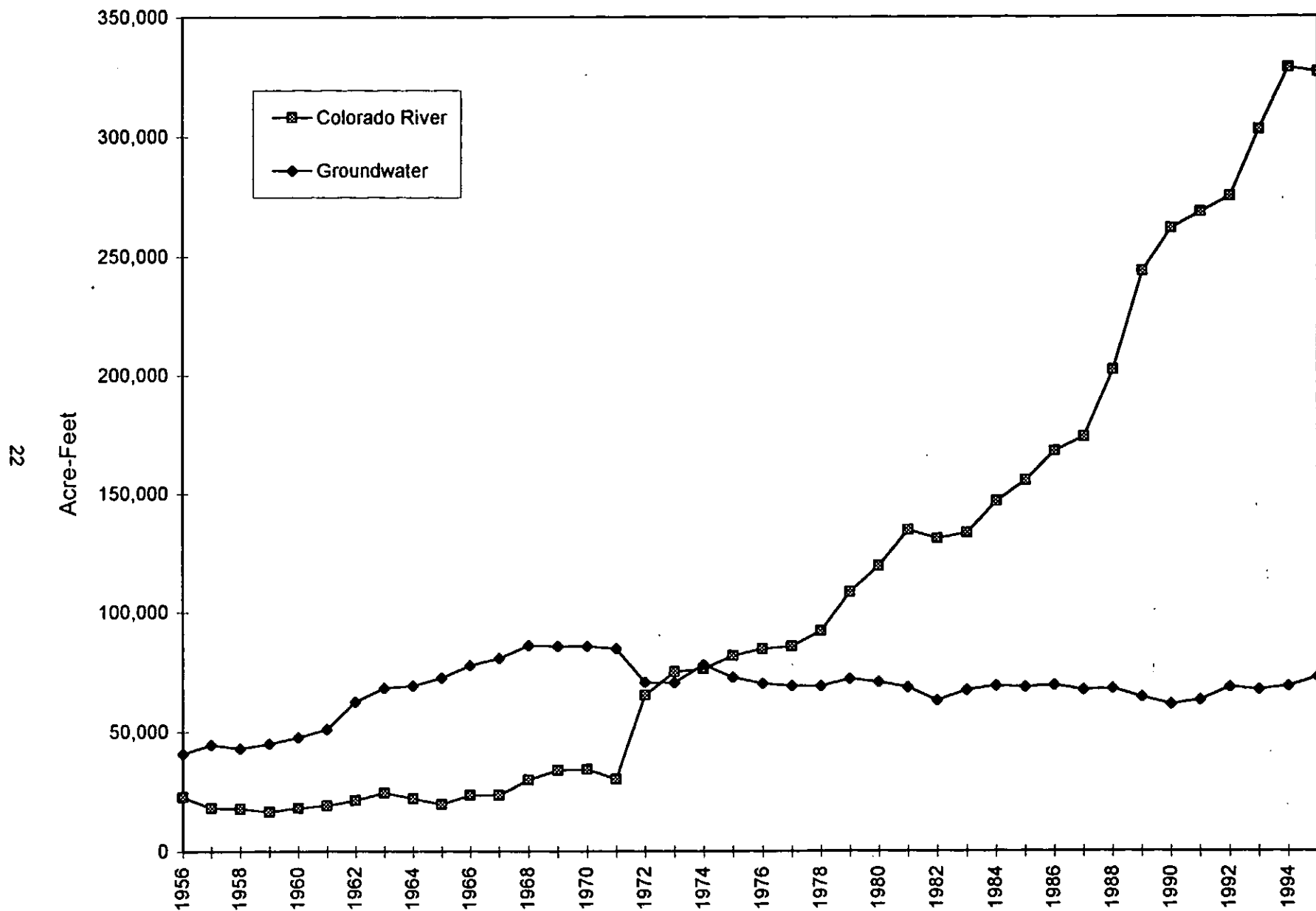
Figure 7. Total groundwater and Colorado River water usage for the Las Vegas Valley, 1956-95.
