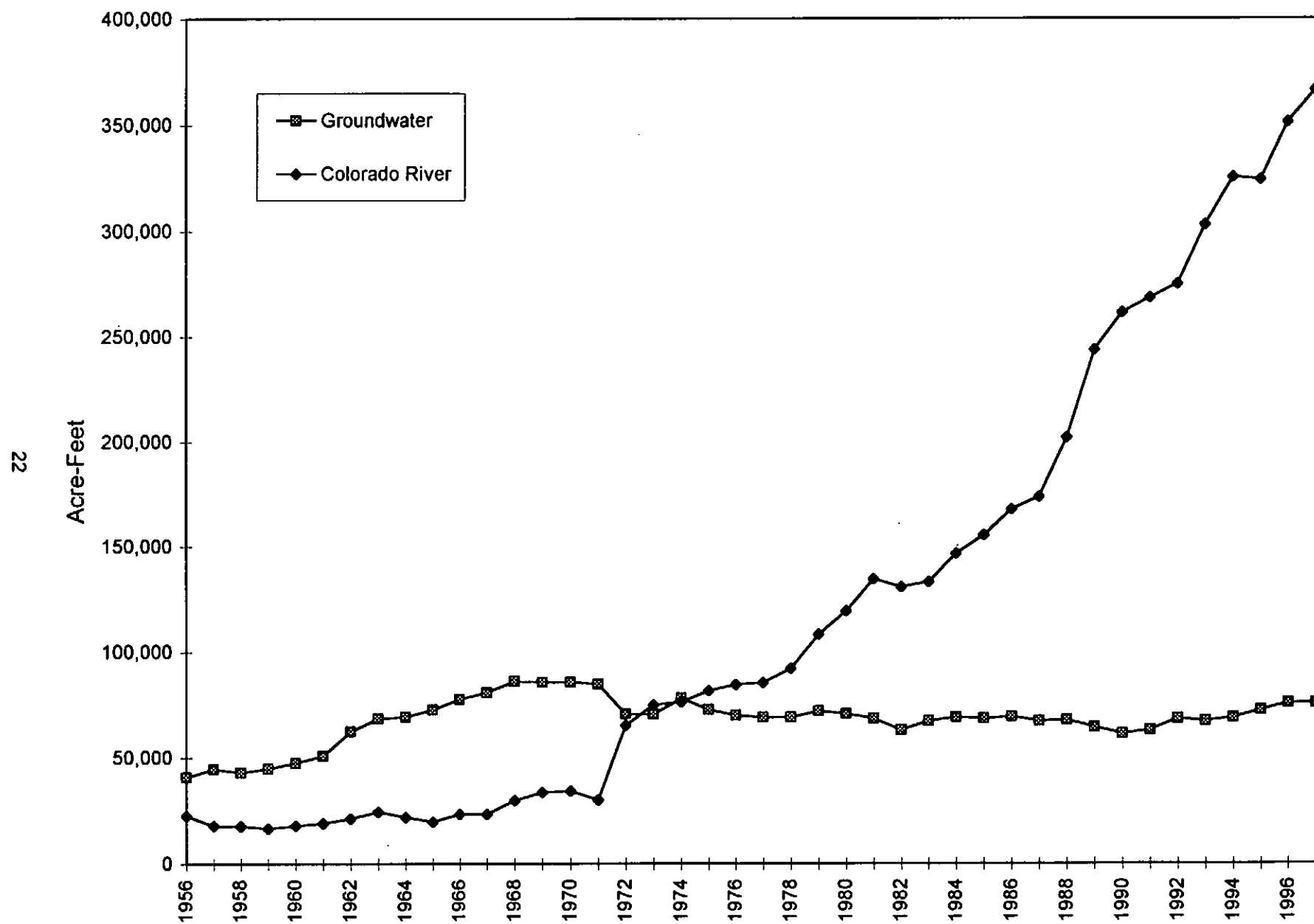
Figure 7. Annual groundwater and Colorado River water usage for the Las Vegas Valley, 1956-97.
