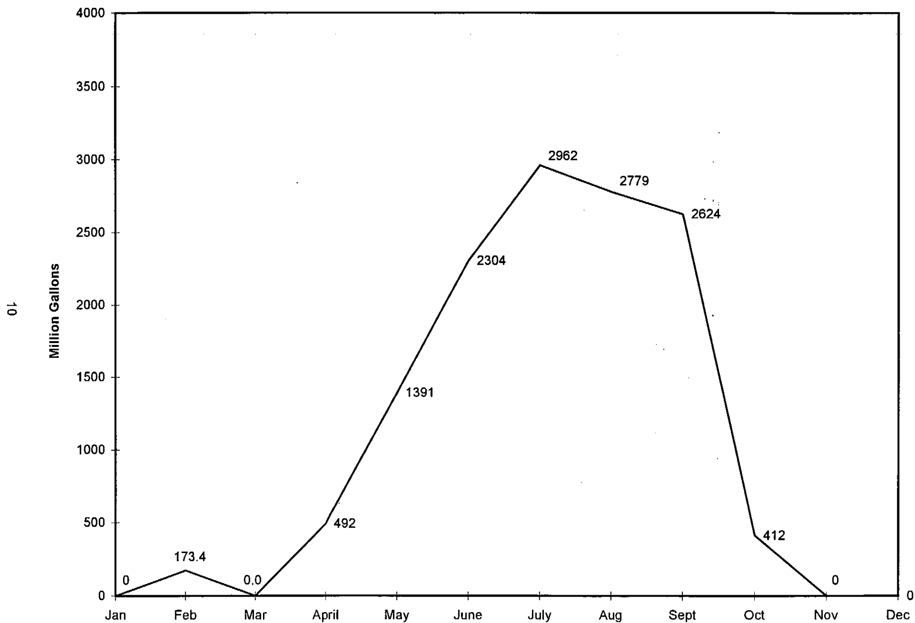
Figure 1. Las Vegas Valley Water District monthly well production for 1997.
