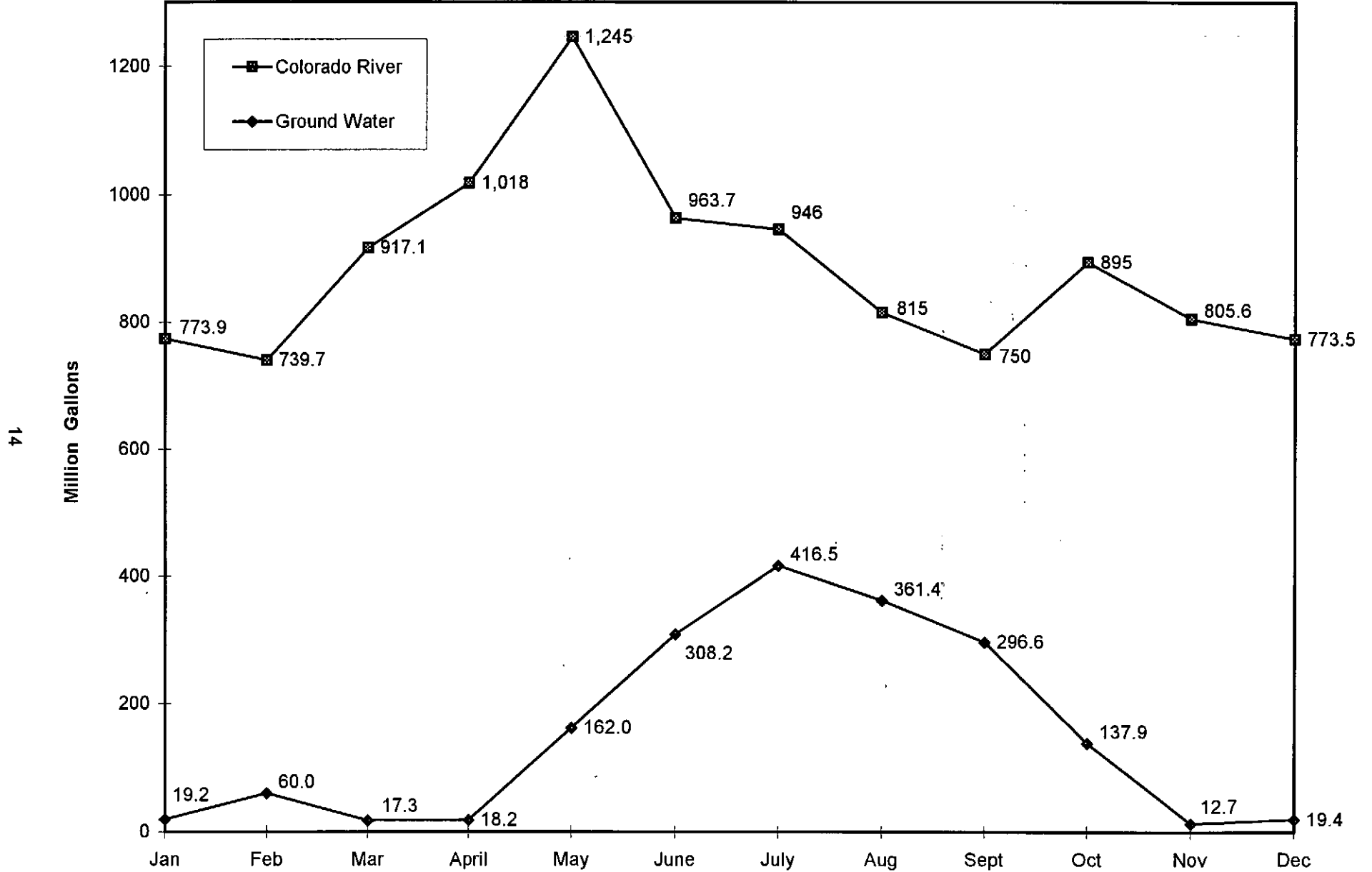
Figure 4. City of North Las Vegas Ground Water and imported Colorado River water usage for 1997.
