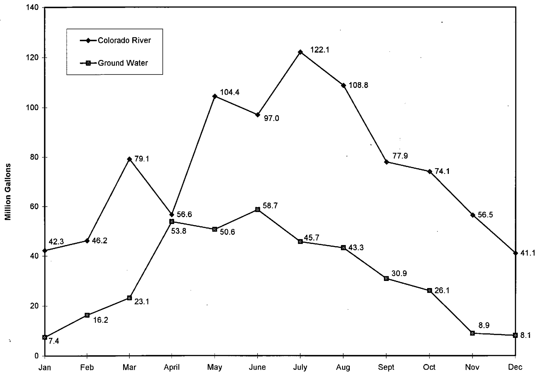
Figure 6. Nellis Air Force Base Ground Water and imported Colorado River water usage for 1997.
