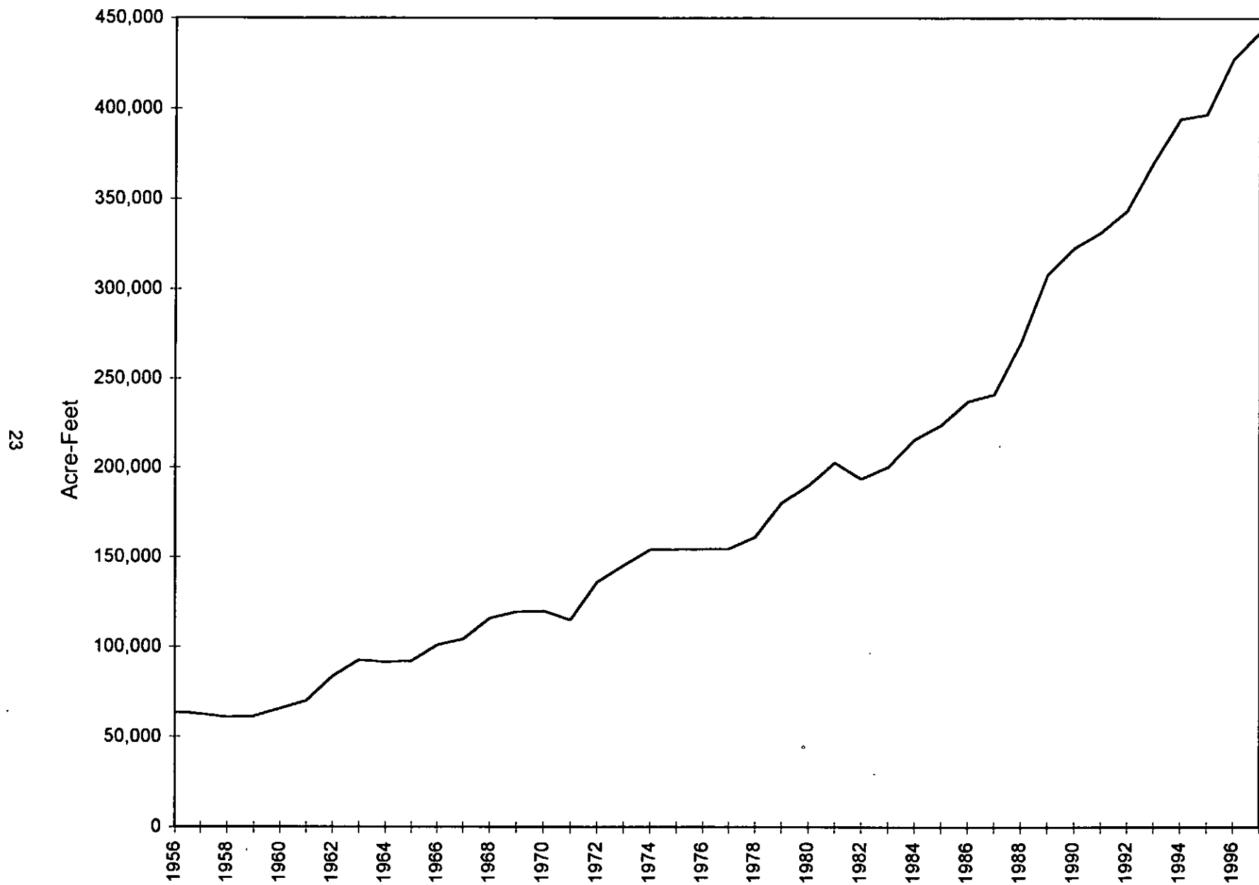
Figure 8. Annual water usage for the Las Vegas Valley, 1956-97.
