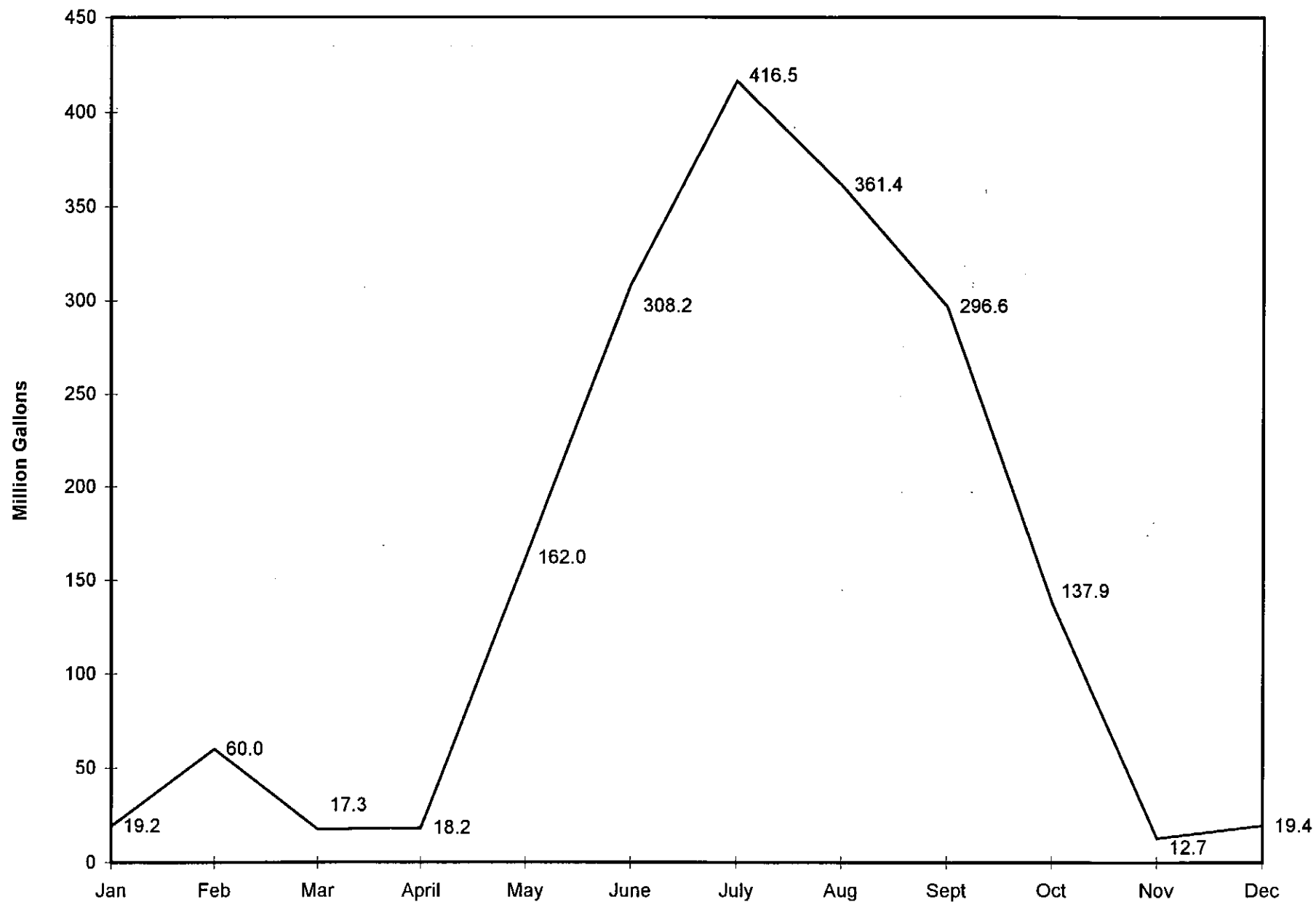
Figure 3. City of North Las Vegas monthly well production for 1997.
