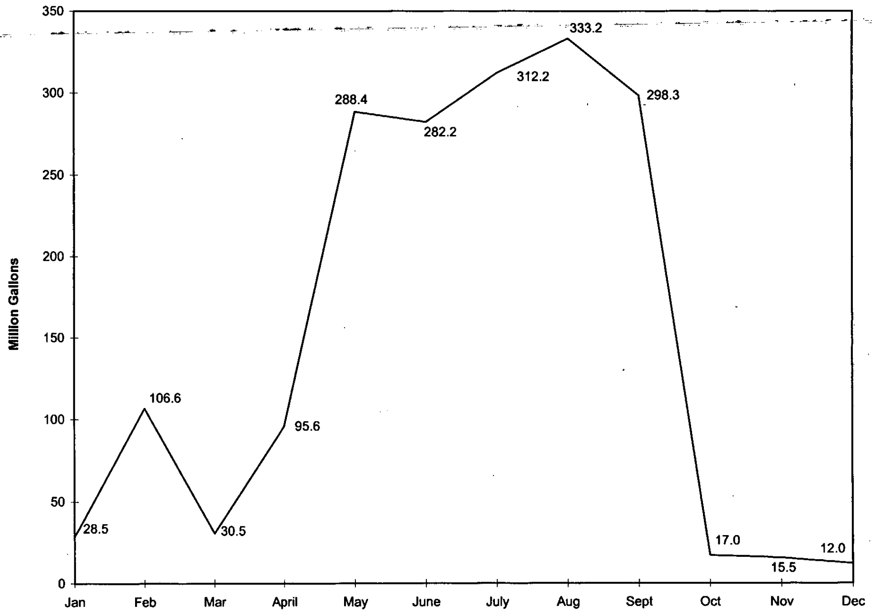
Figure 3. City of North Las Vegas monthly well production for 2002.
