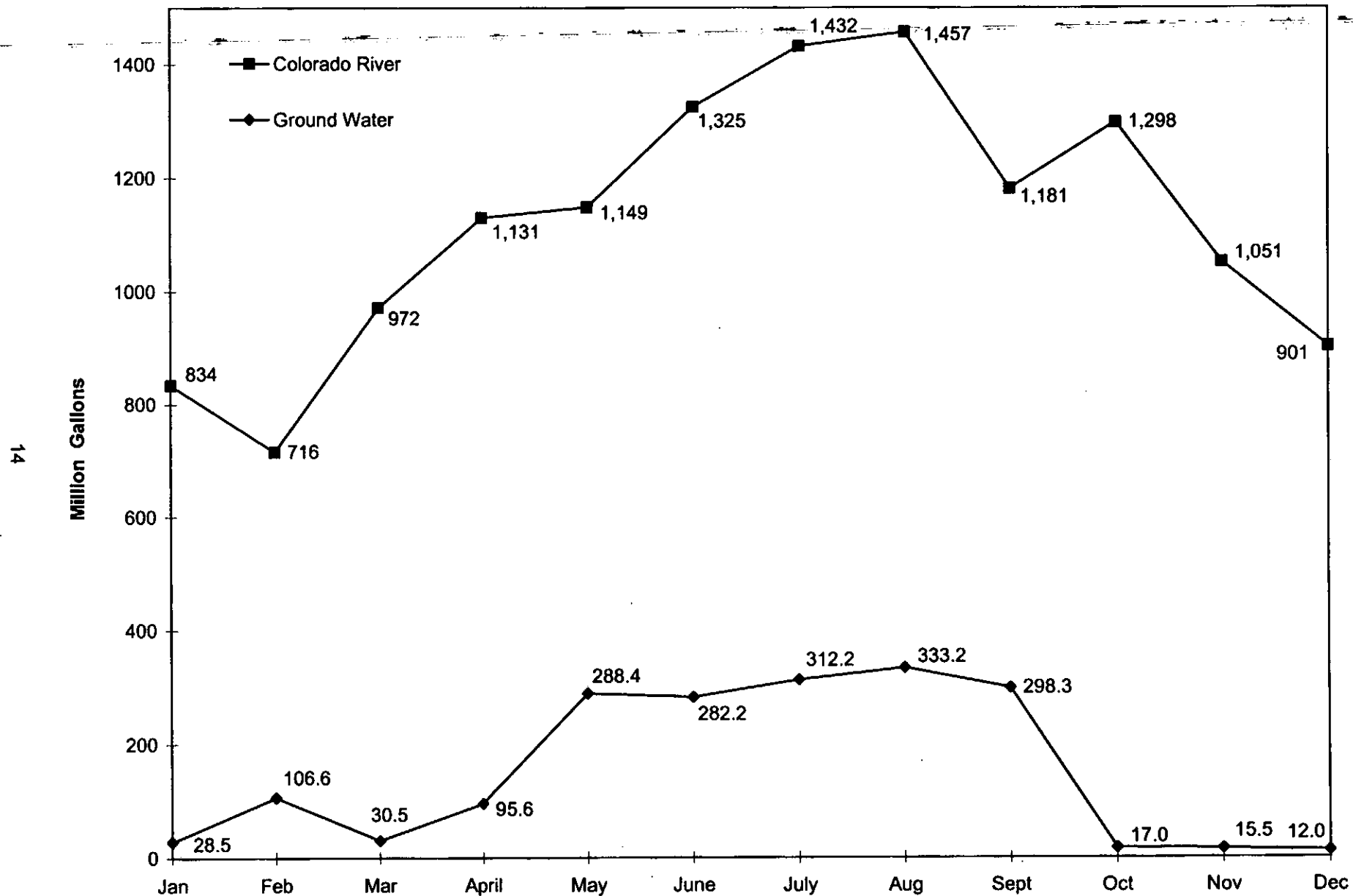
Figure 4. City of North Las Vegas Ground Water and imported Colorado River water usage for 2002.
