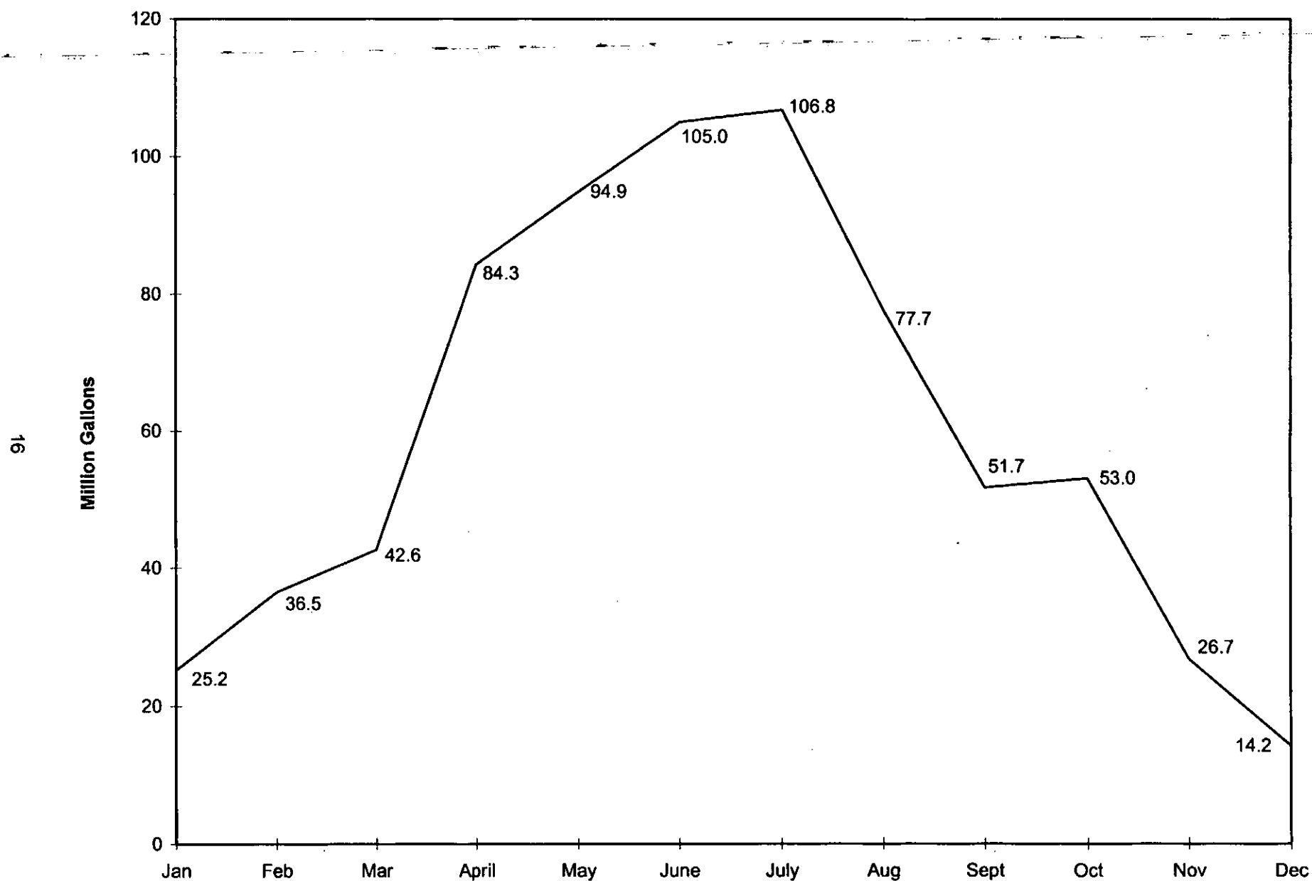
Figure 5. Nellis Air Force Base monthly well production for 2002.
