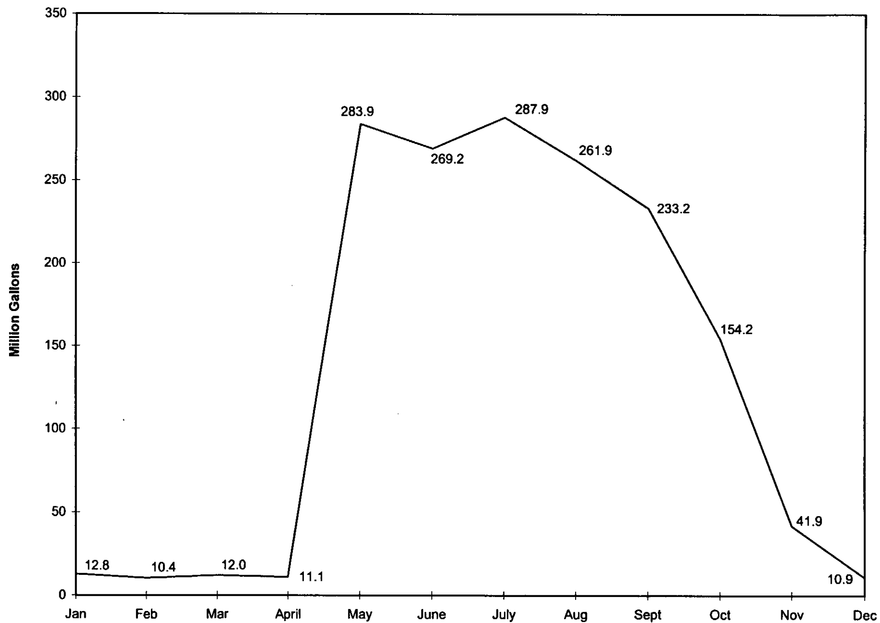
Figure 3. City of North Las Vegas monthly well production for 2003.
