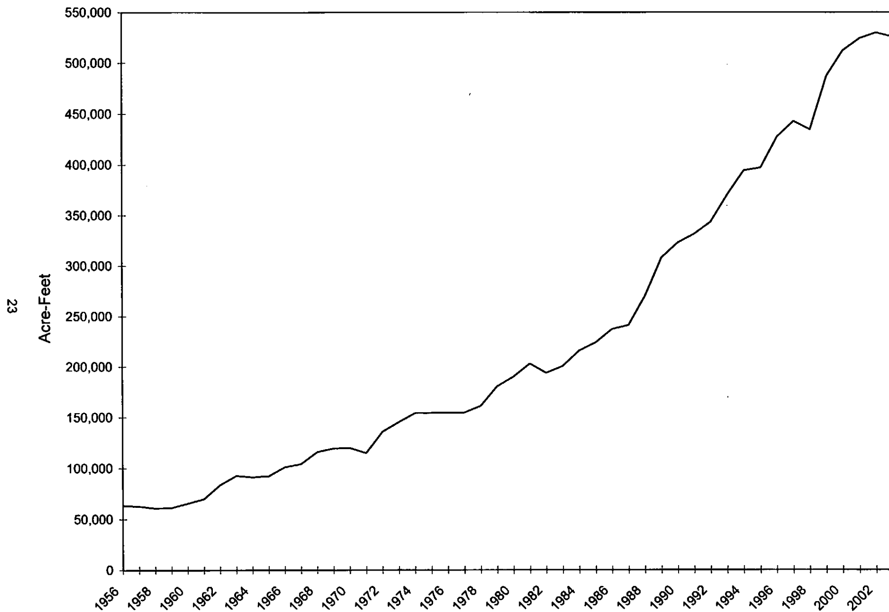
Figure 8. Annual water usage for the Las Vegas Valley, 1956-03.
