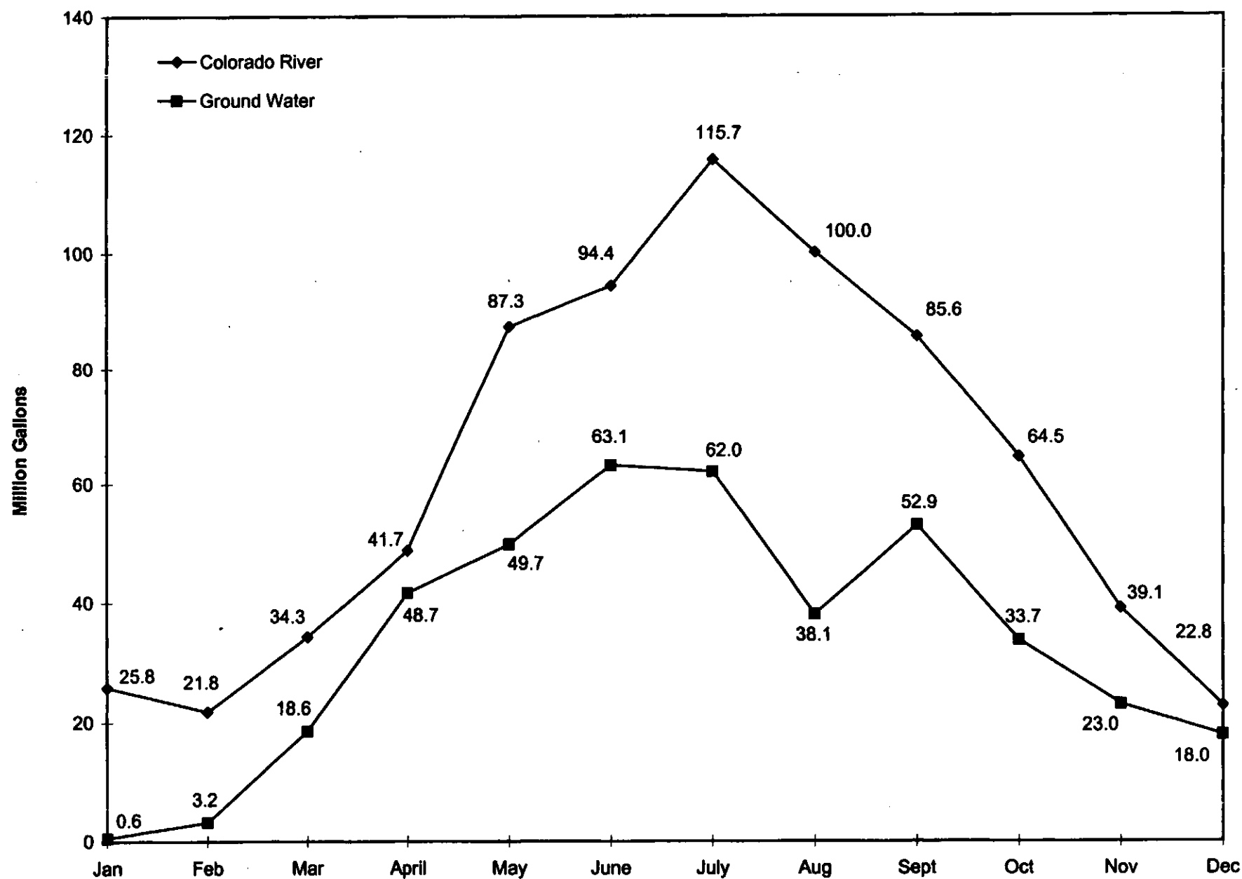
Figure 6. Nellis Air Force Base Ground Water and Imported Colorado River water usage for 2005.
