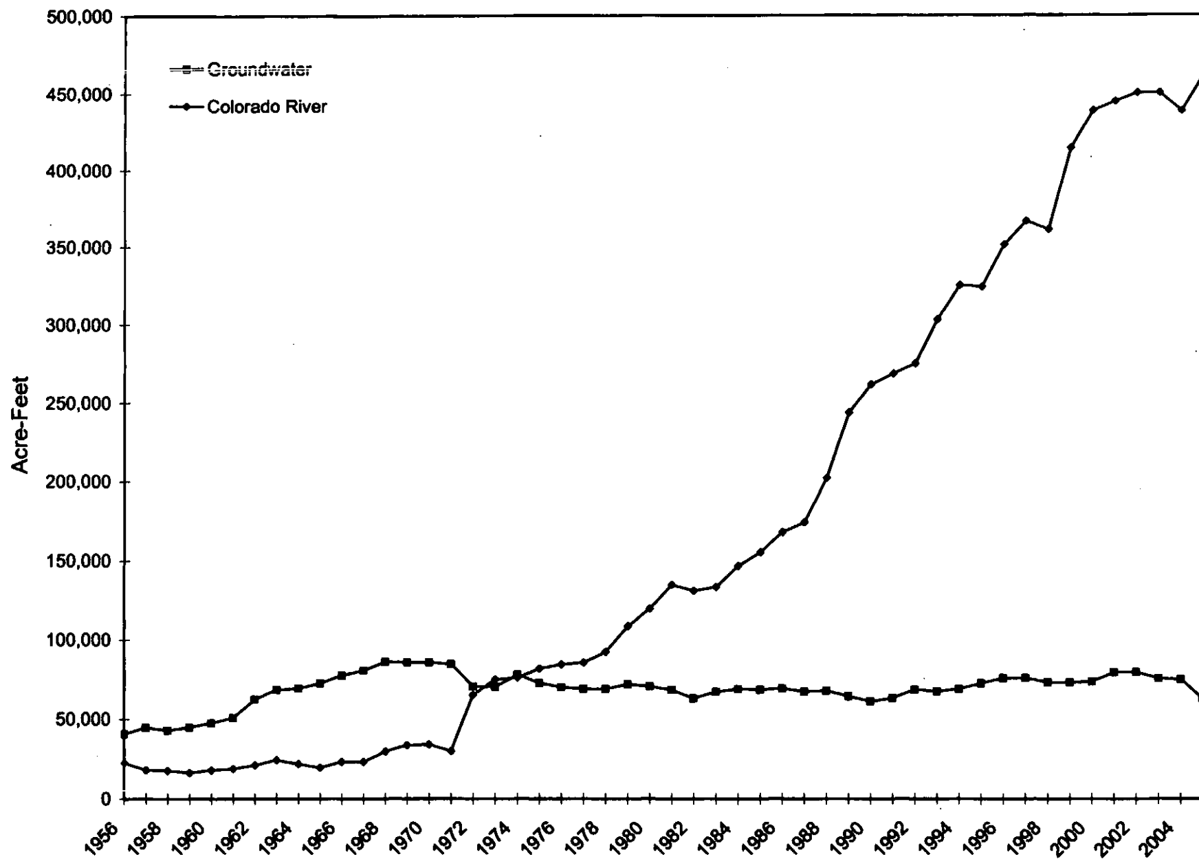
Figure 7. Annual groundwater and Colorado River water usage for the Las Vegas Valley, 1956-05.
