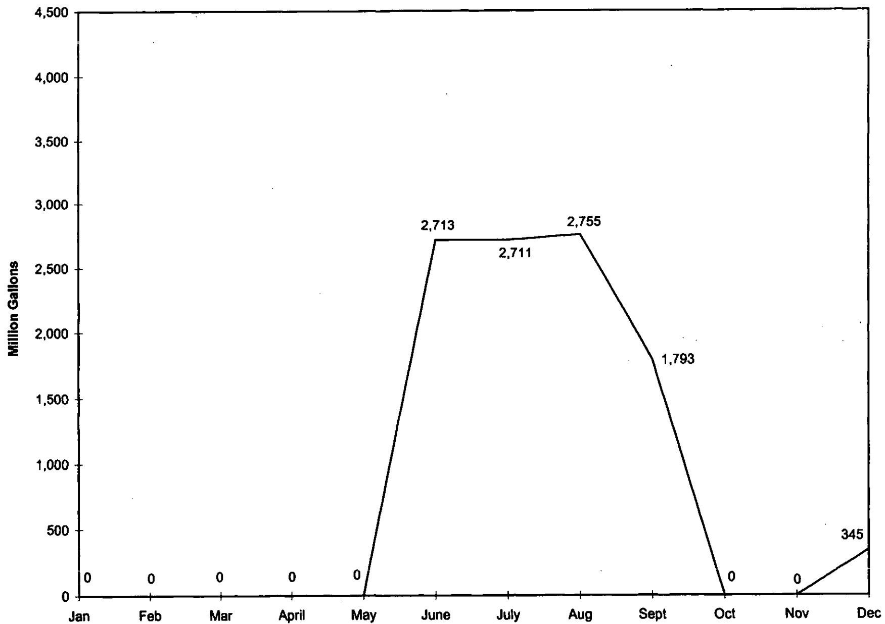
Figure 1. Las Vegas Valley Water District monthly well production for 2005.
