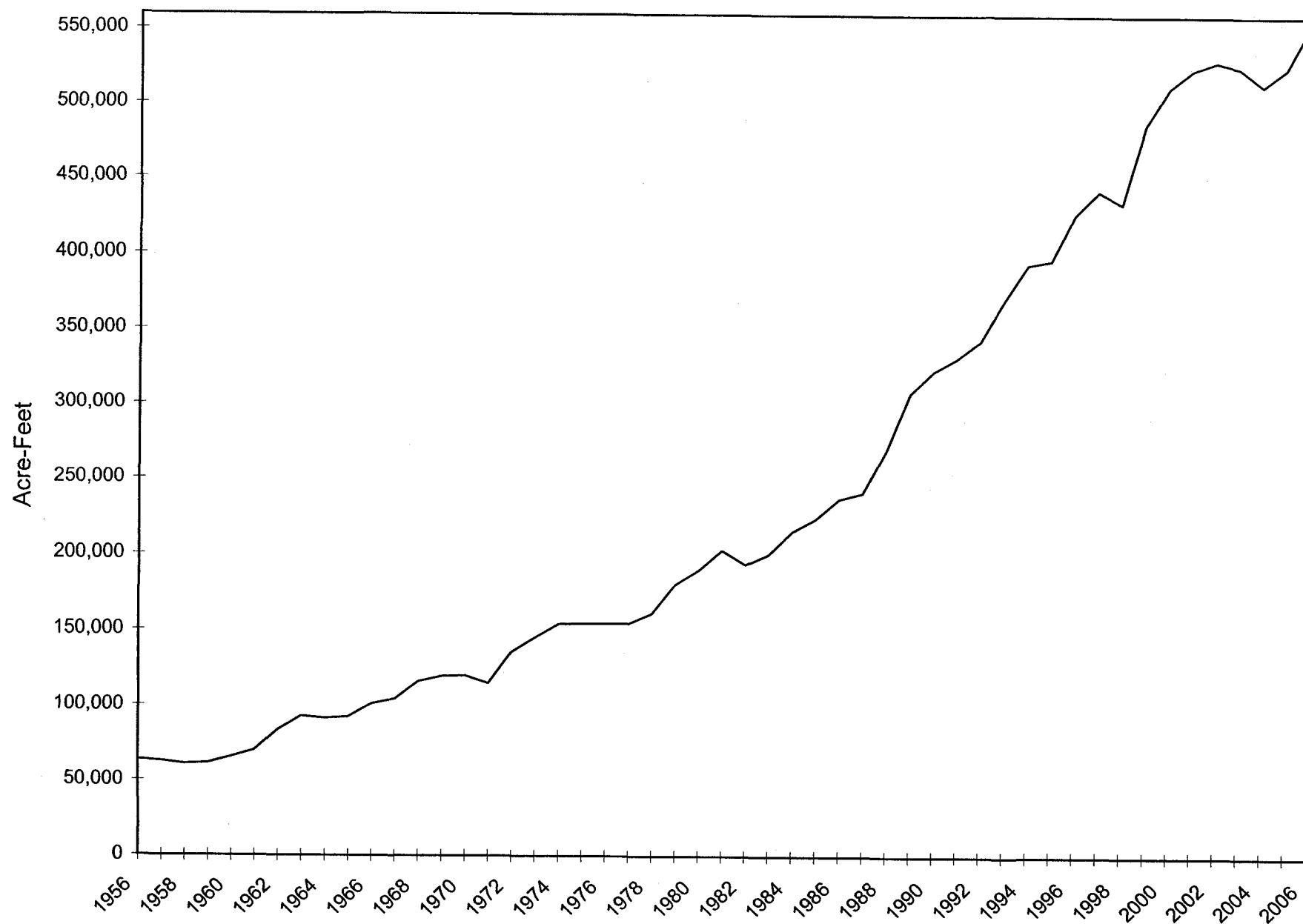
Figure 8. Annual water usage for the Las Vegas Valley, 1956-06.
