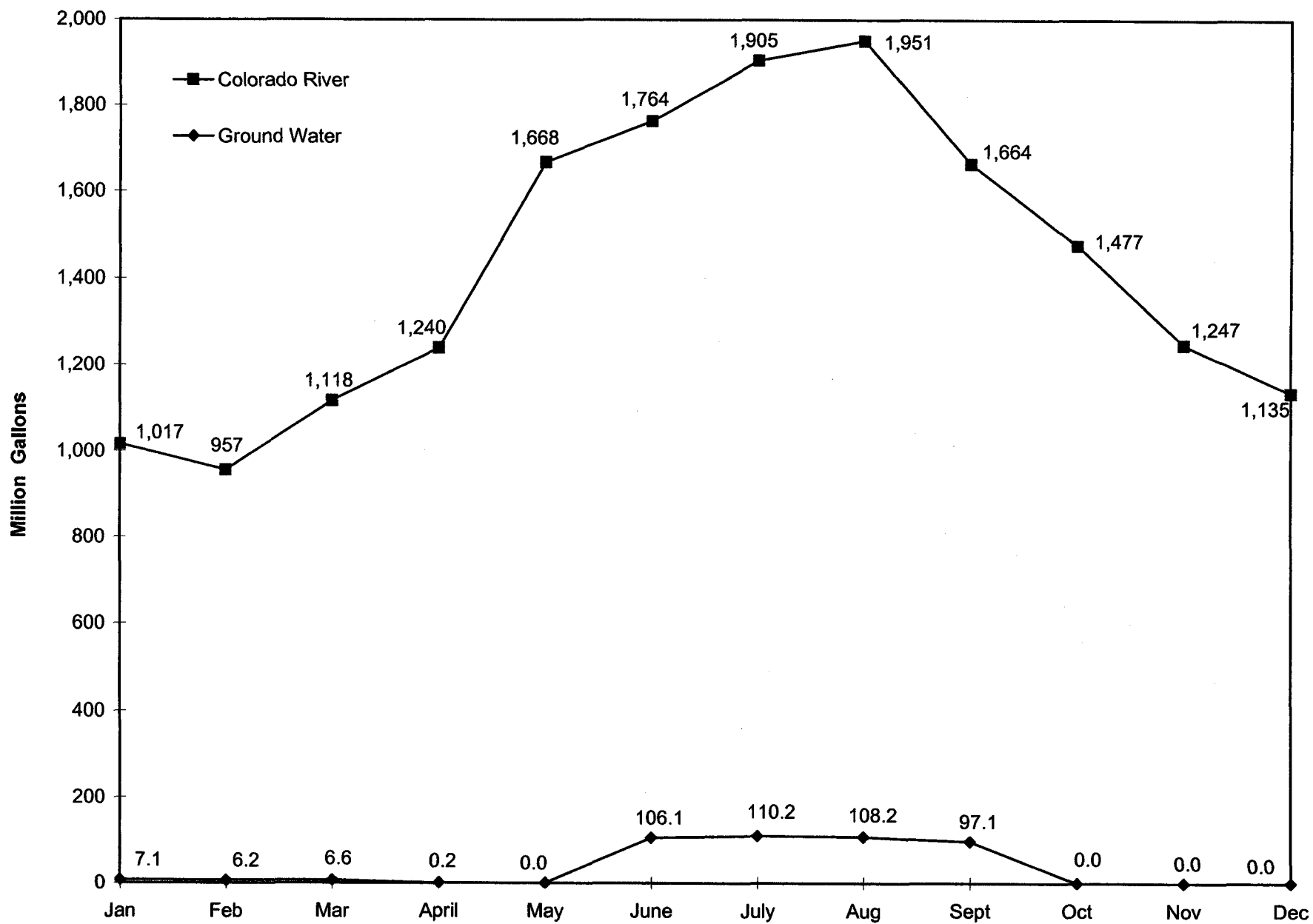
Figure 4. City of North Las Vegas Ground Water and imported Colorado River water usage for 2006.
