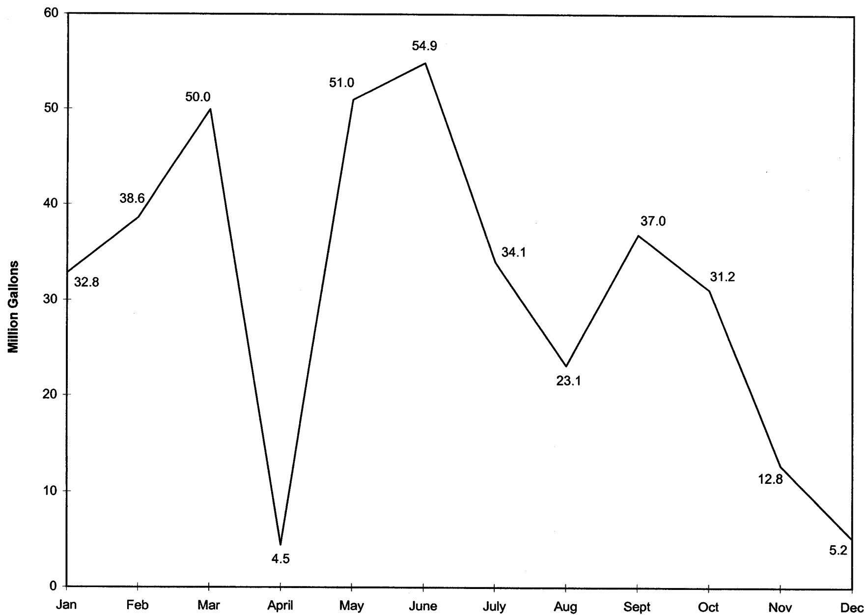
Figure 5. Nellis Air Force Base monthly well production for 2006.
