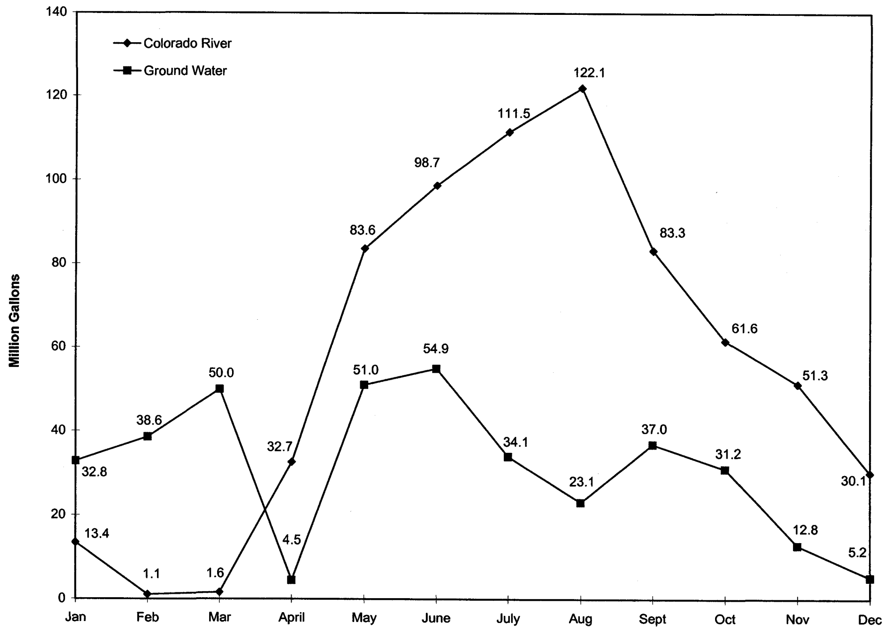
Figure 6. Nellis Air Force Base Ground Water and imported Colorado River water usage for 2006.
