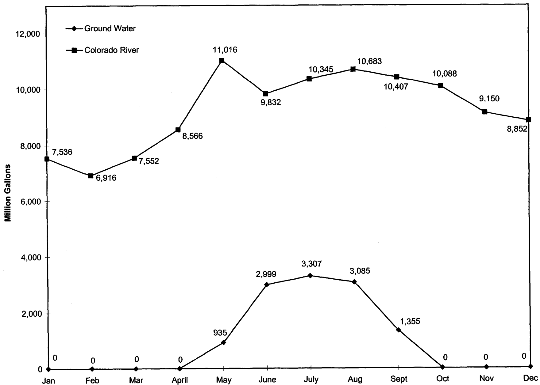
Figure 2. Las Vegas Valley Water District Ground Water and imported Colorado River water usage for 2006.
