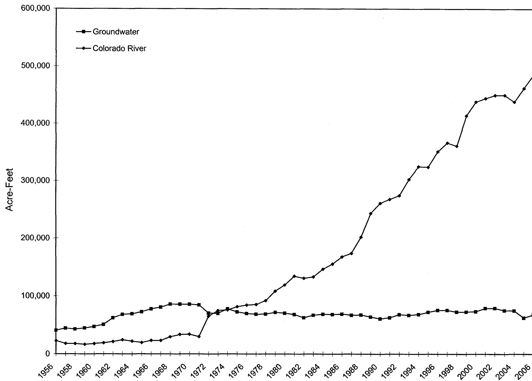
Figure 7. Annual groundwater and Colorado River water usage for the Las Vegas Valley, 1956-06.
