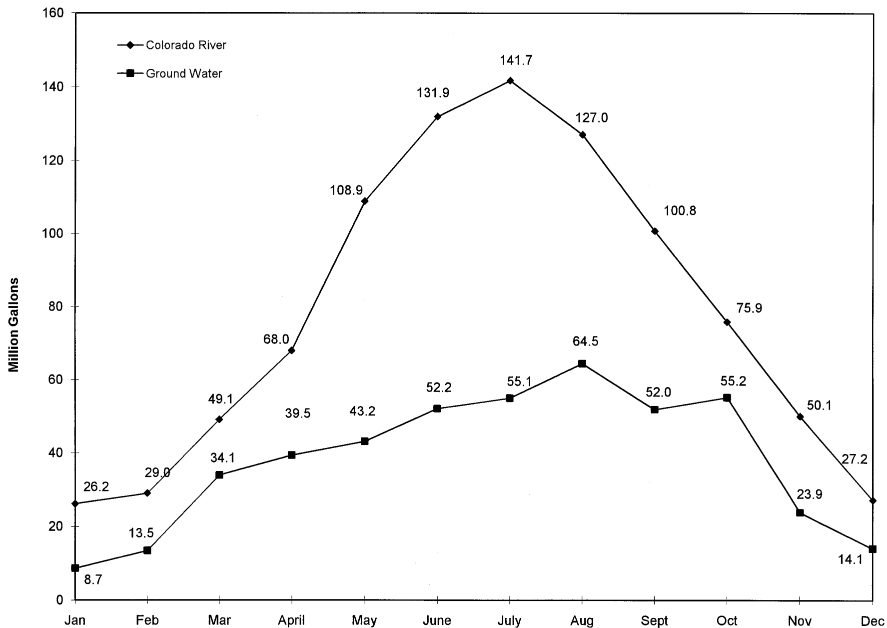
Figure 6. Nellis Air Force Base Ground Water and imported Colorado River water usage for 2007.
