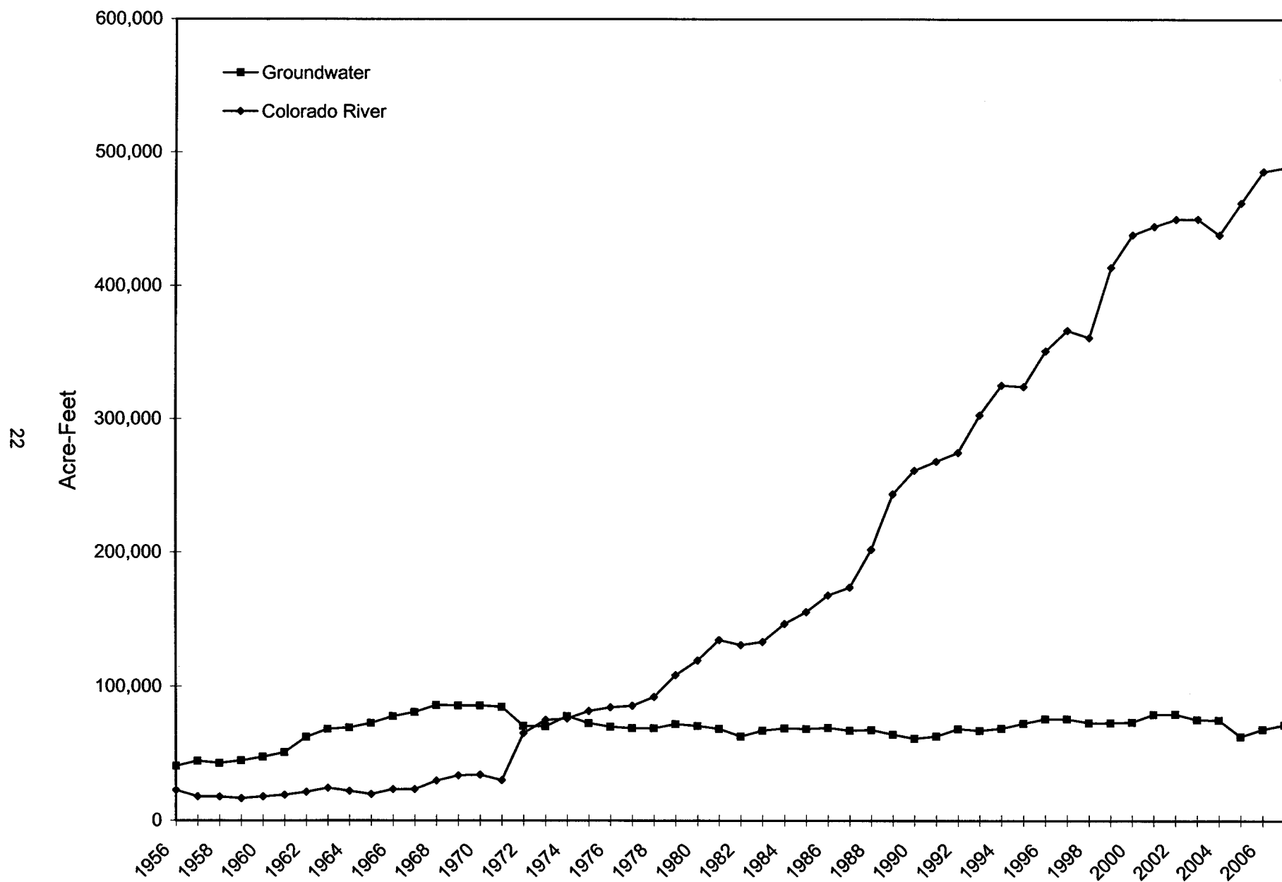
Figure 7. Annual groundwater and Colorado River water usage for the Las Vegas Valley, 1956-07.
