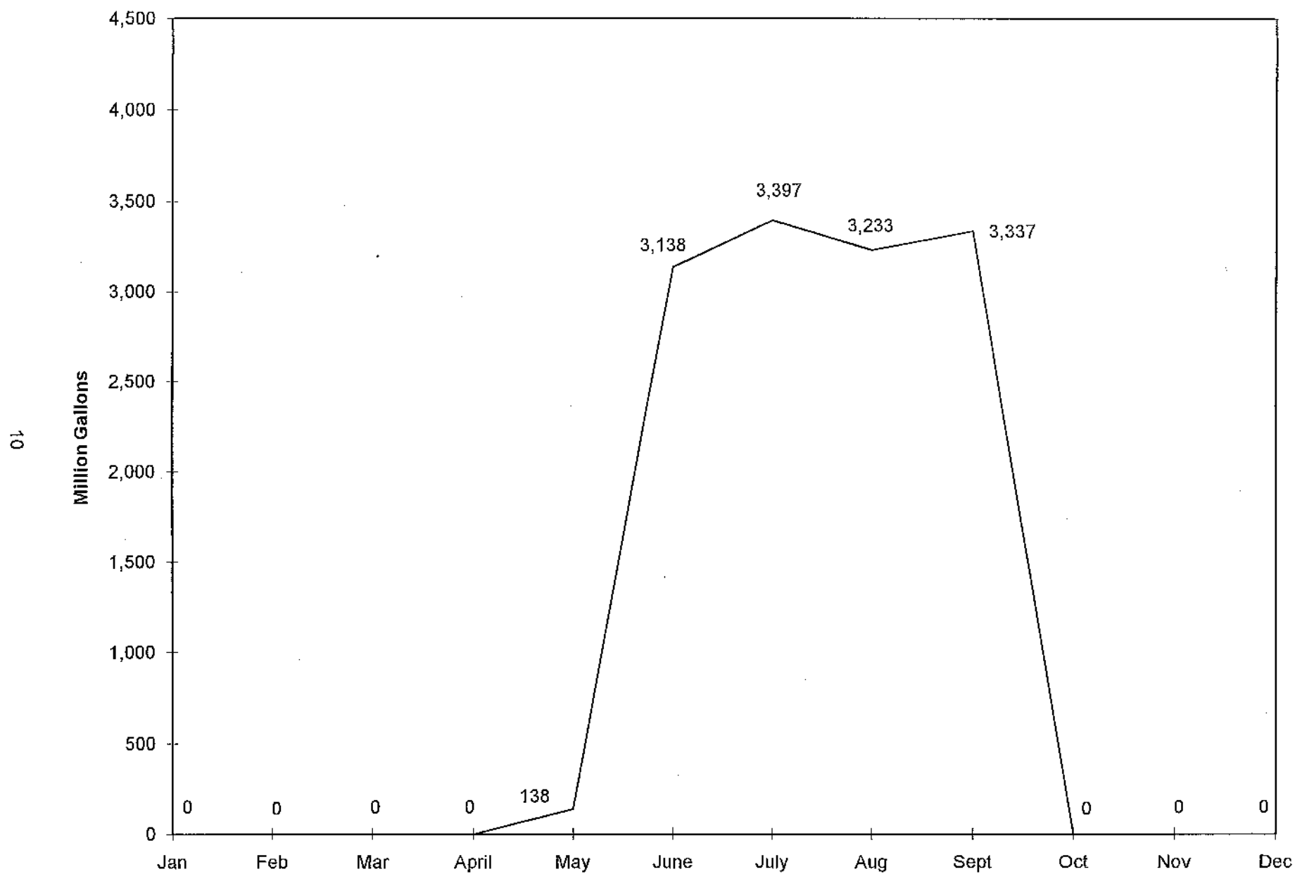
Figure 1. Las Vegas Valley Water District monthly well production for 2009.
