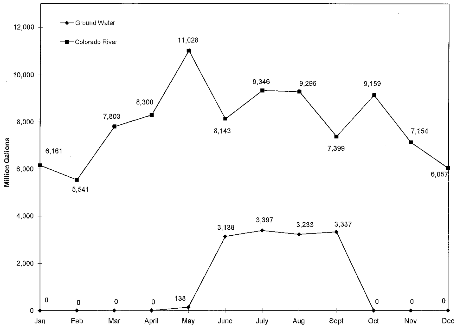
Figure 2. Las Vegas Valley Water District Ground Water and imported Colorado River water usage for 2009.
