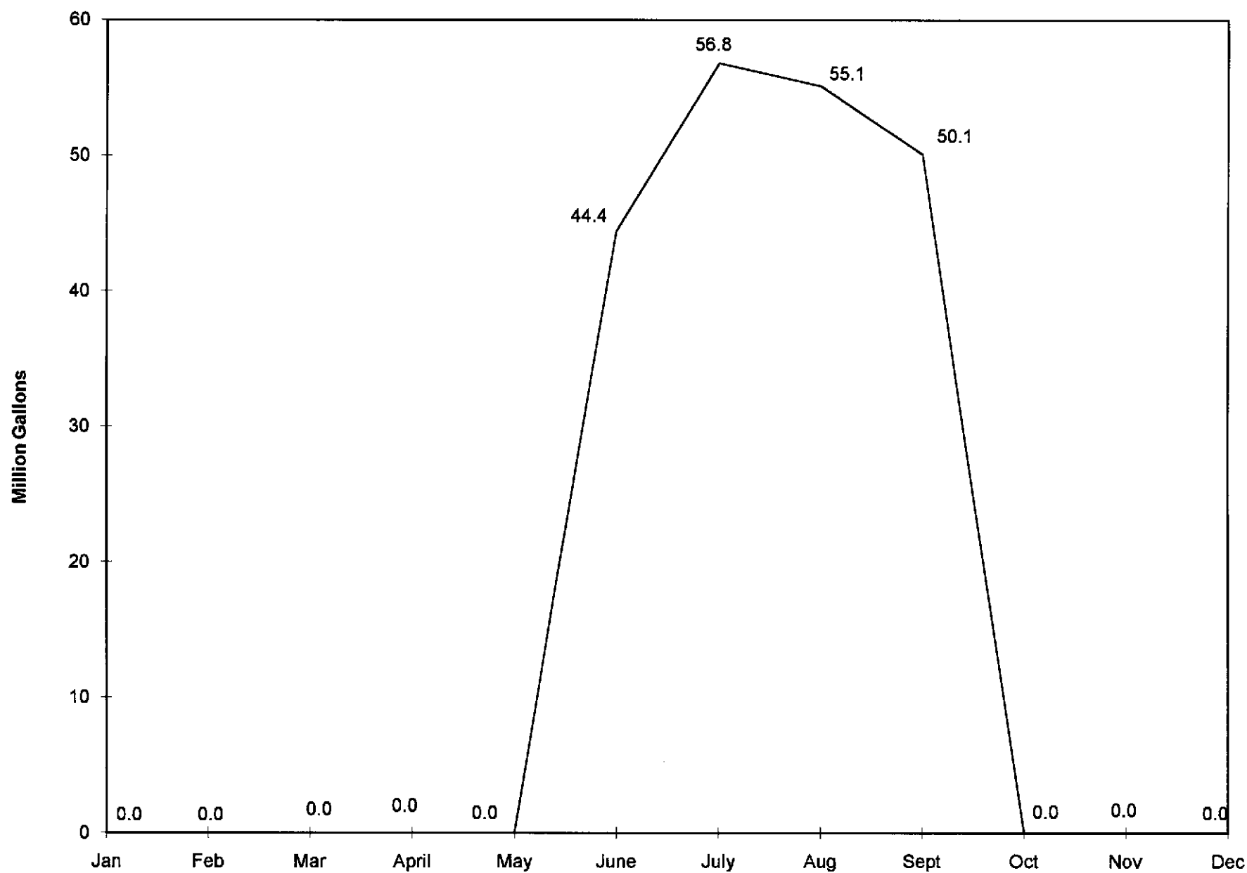
Figure 3. City of North Las Vegas monthly well production for 2010.
