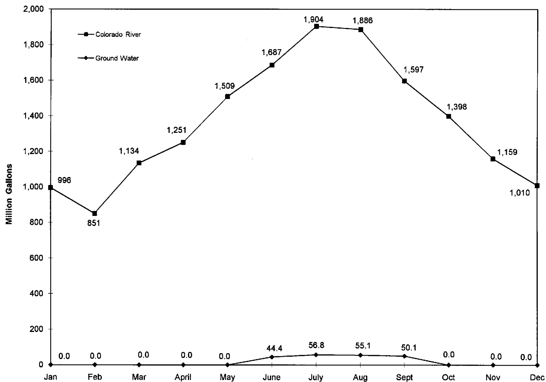
Figure 4. City of North Las Vegas Ground Water and imported Colorado River water usage for 2010.
