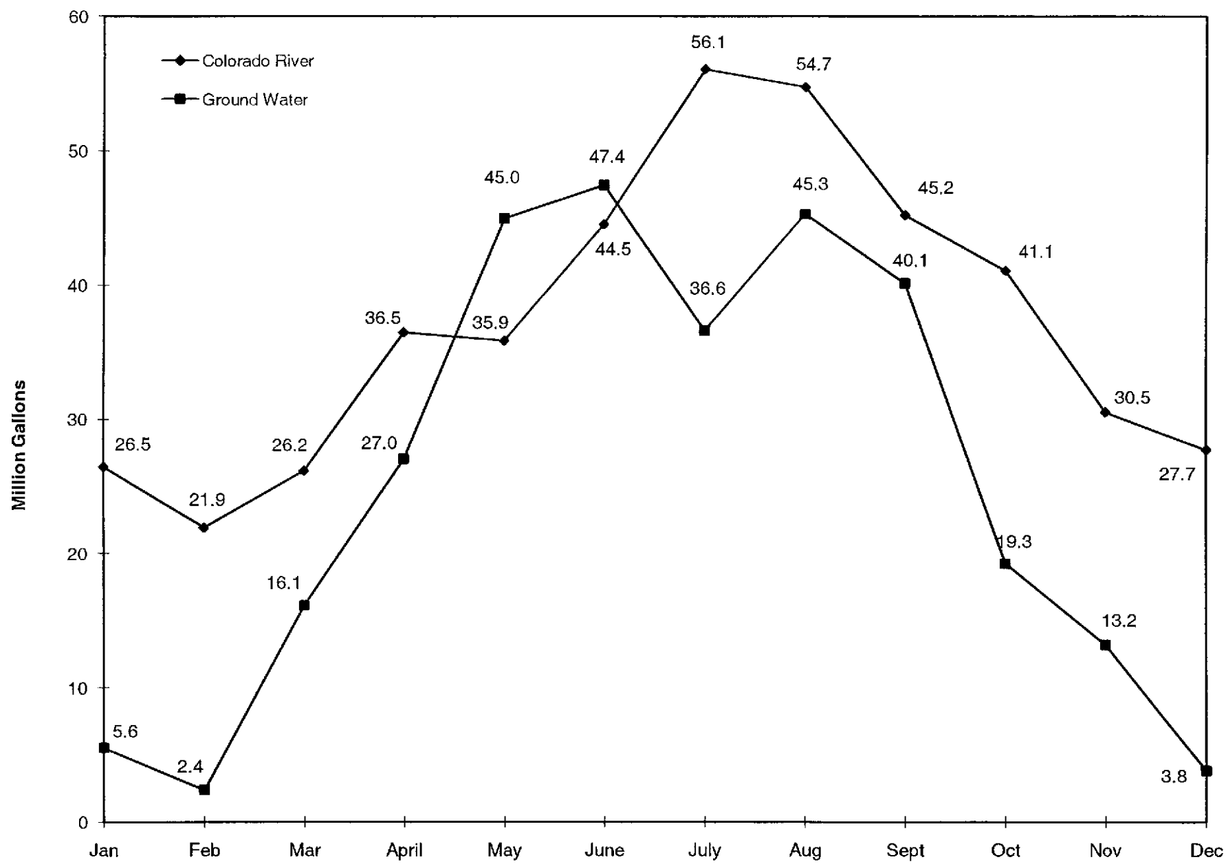
Figure 6. Nellis Air Force Base Ground Water and imported Colorado River water usage for 2010.
