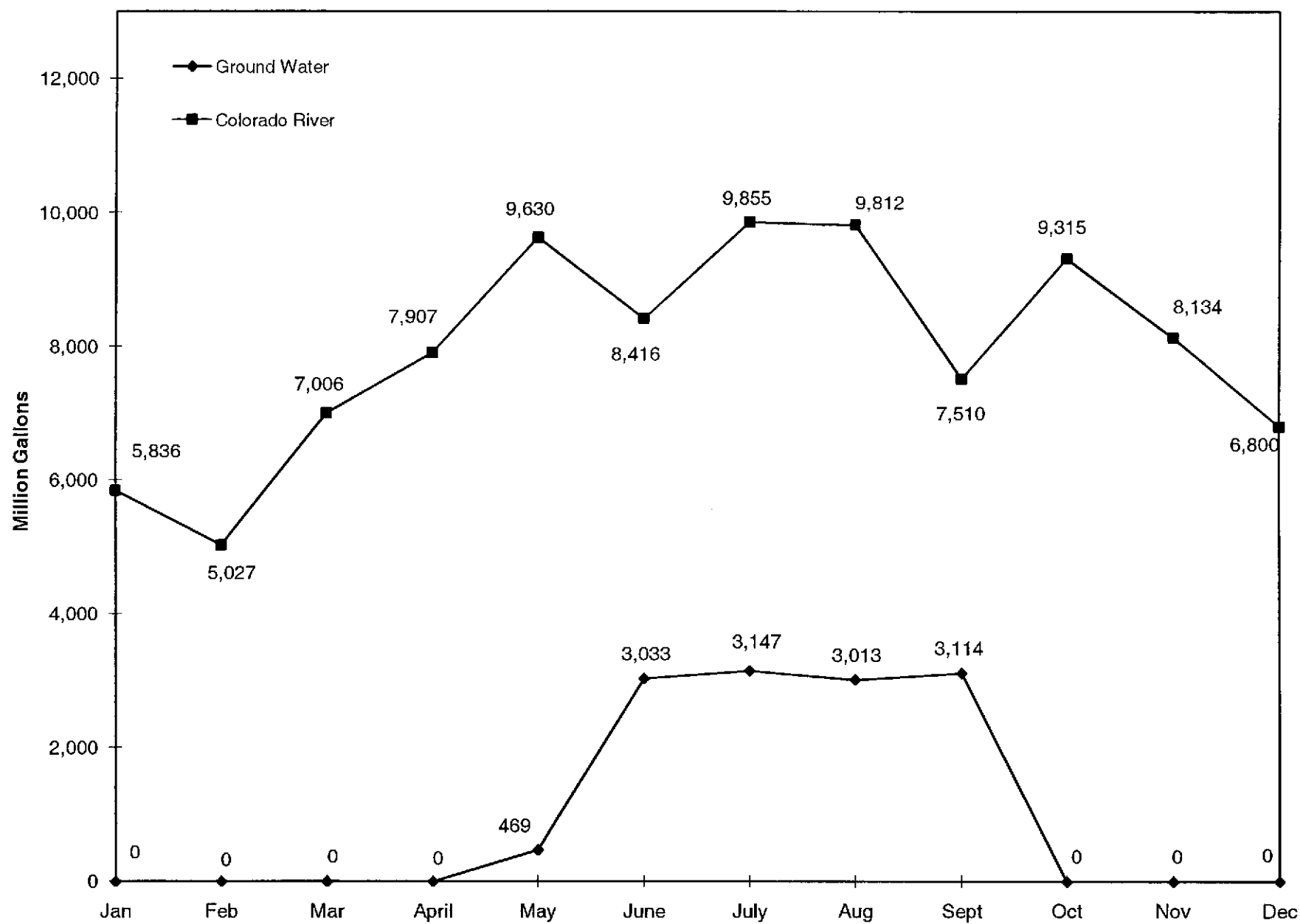
Figure 2. Las Vegas Valley Water District Ground Water and imported Colorado River water usage for 2010.
