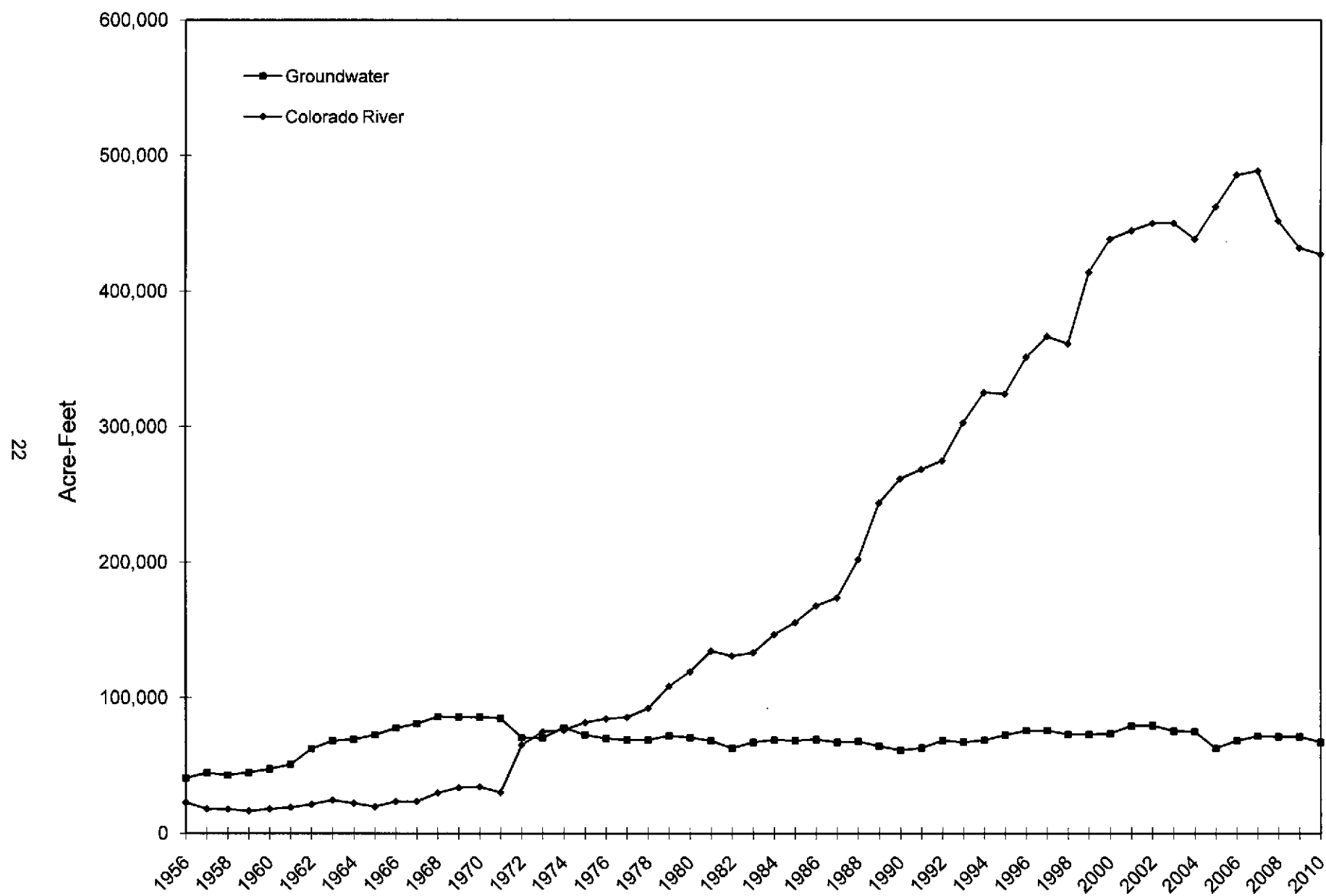
Figure 7. Annual groundwater and Colorado River water usage for the Las Vegas Valley, 1956-2010
