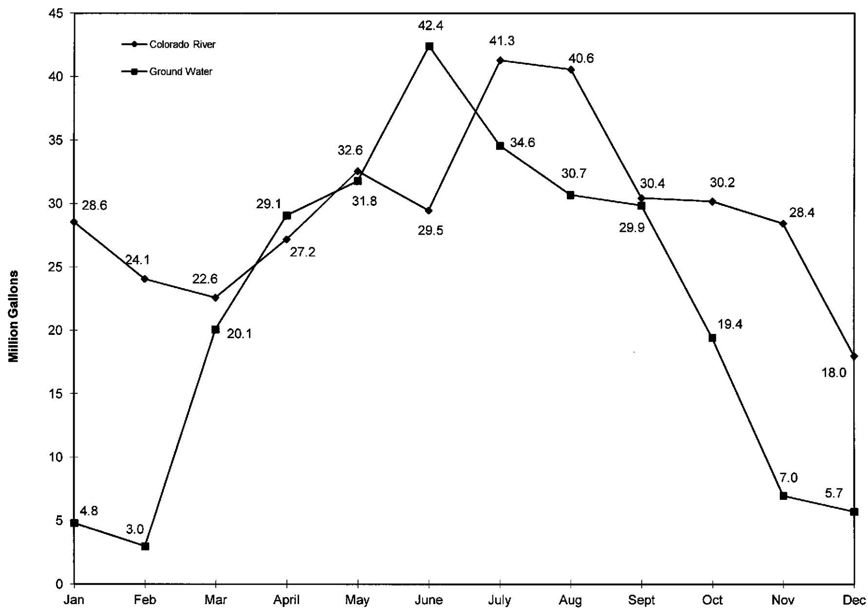
Figure 6. Nellis Air Force Base Ground Water and imported Colorado River water usage for 2013.
