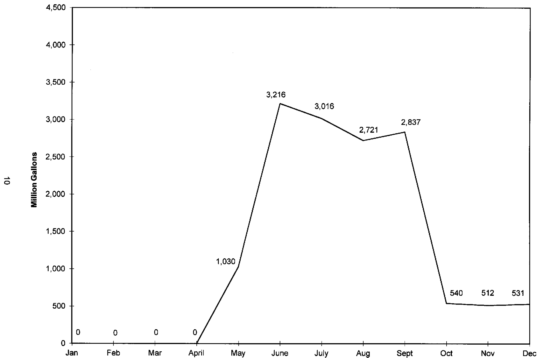
Figure 1. Las Vegas Valley Water District monthly well production for 2013.
