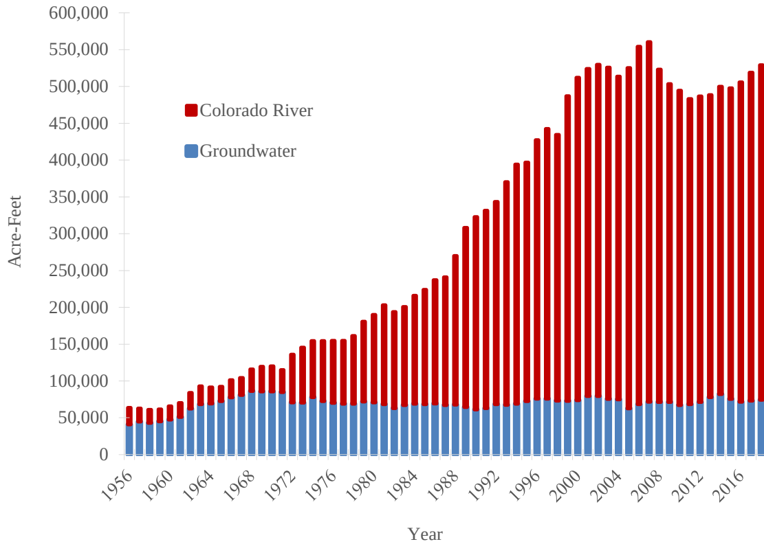
Figure 3. Total annual groundwater and imported Colorado River water usage 1956-2018.
