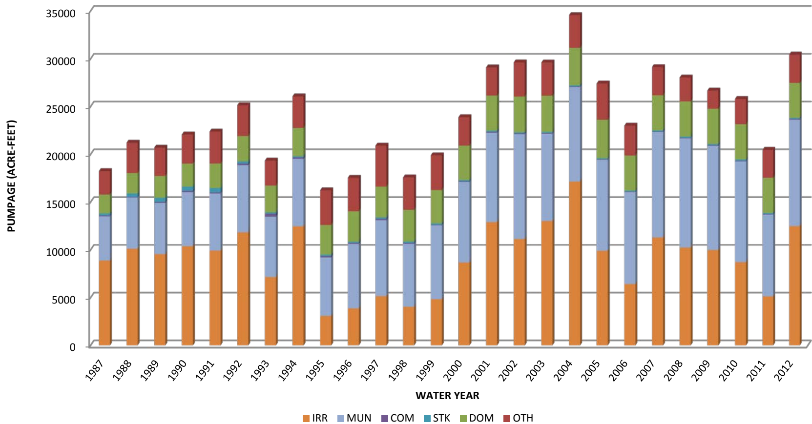
Figure 7. Carson Valley groundwater pumpage variation by water year and manner of use. Includes claims of vested right and pumpage from domestic wells.
