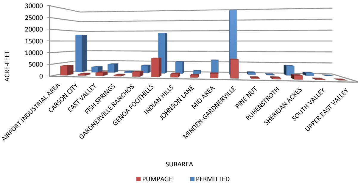
Figure 5. Carson Valley groundwater use permitted and pumped by subarea.
