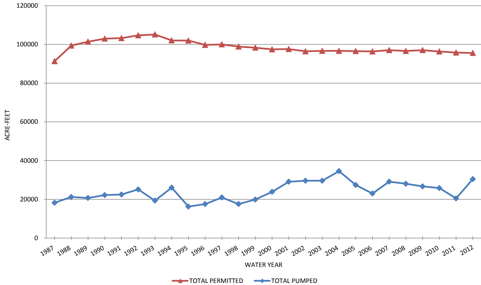
Figure 9. Comparison between permitted and pumped Carson Valley groundwater by water year.
