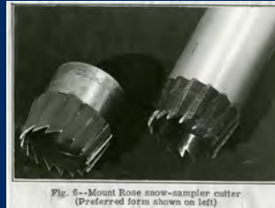
A close-up of the serrated end of the Mt. Rose snow sampler cutter.
